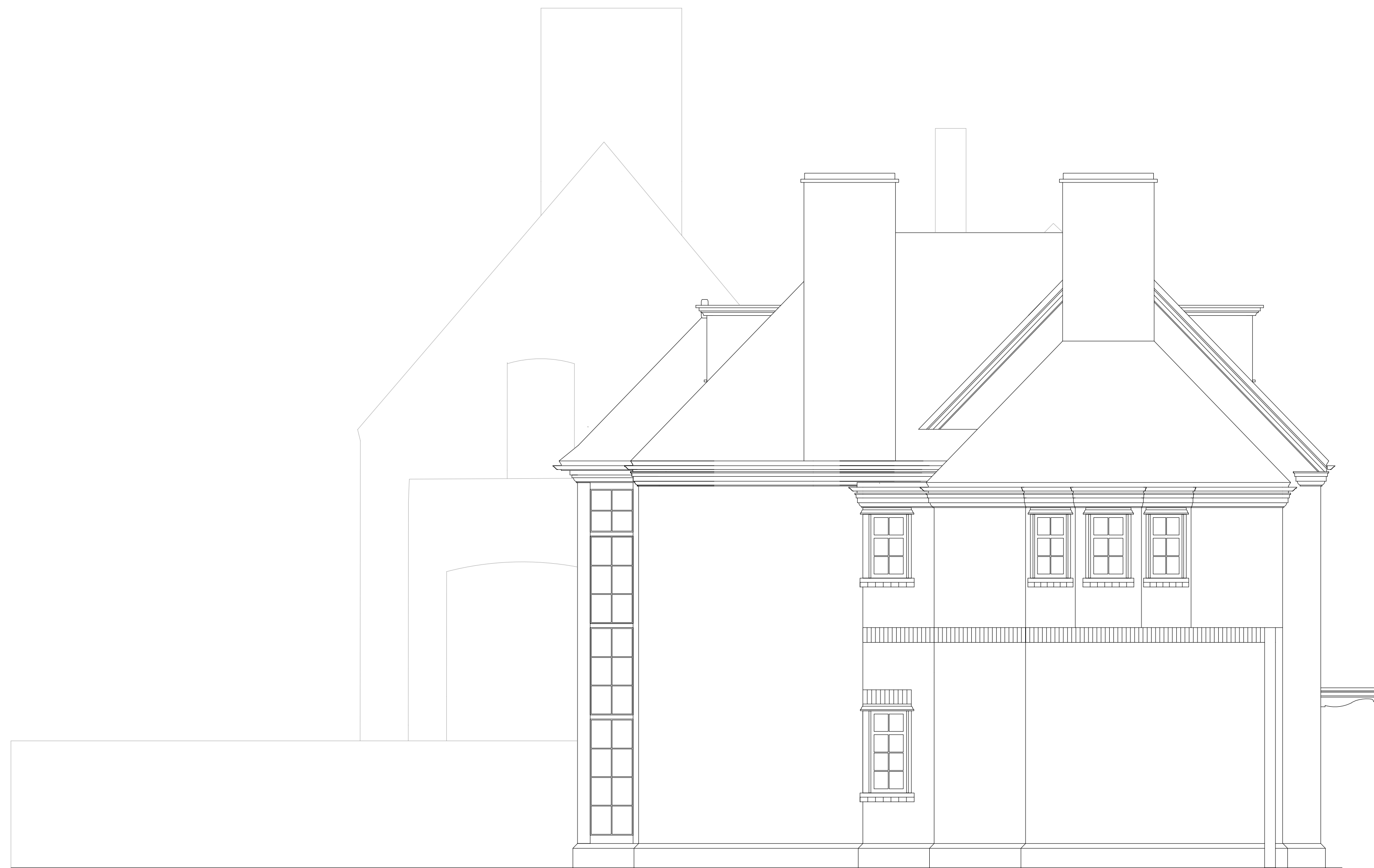
1 Proposed Side Elevation - East Scale: 1:50
