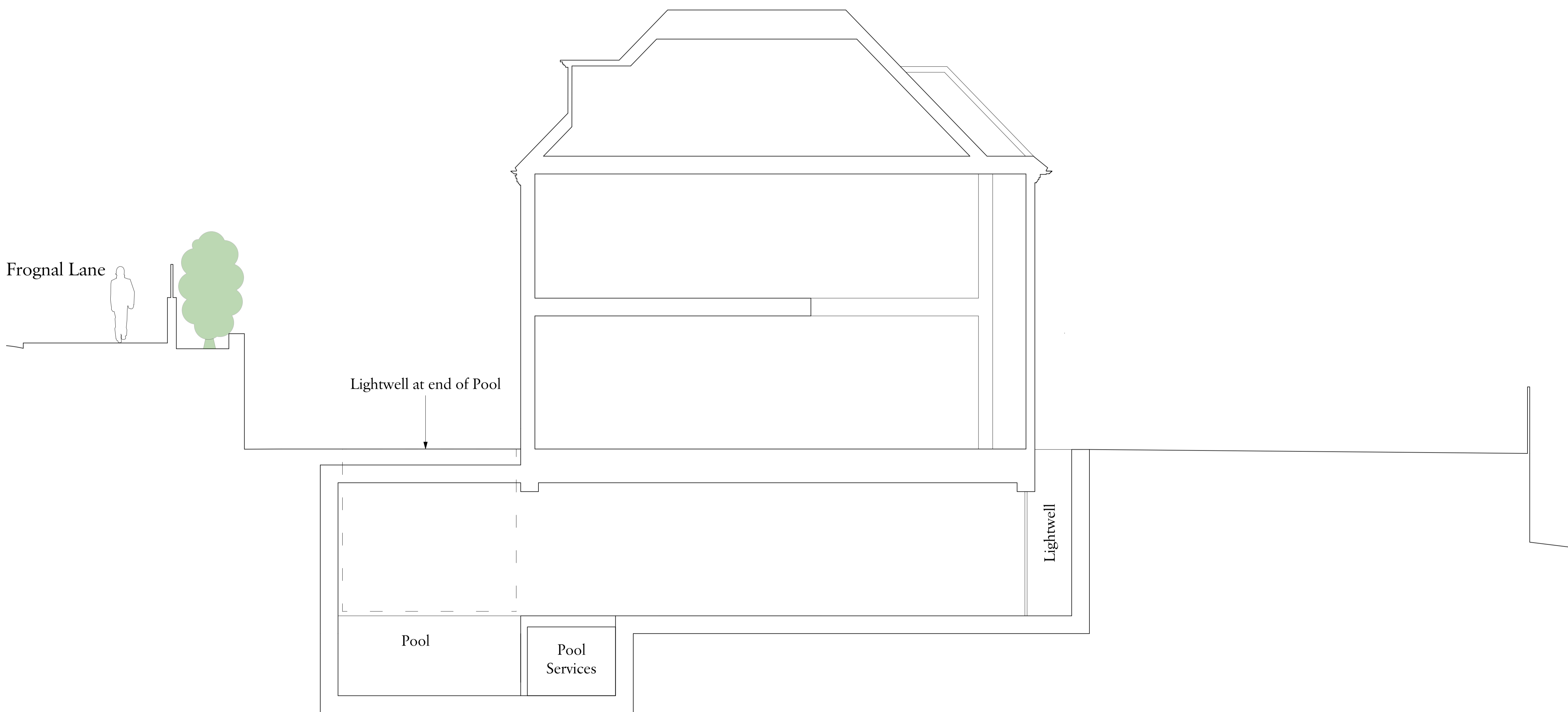
1 Proposed Section - BB Scale: 1:50
