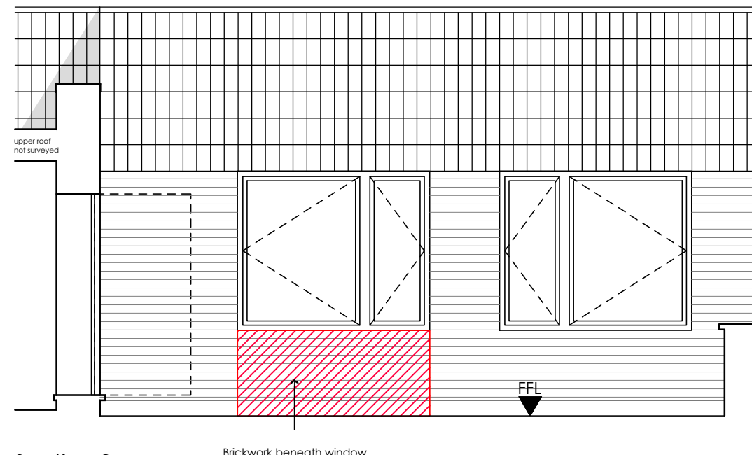
Section 2
