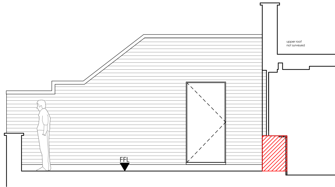
Section 1
