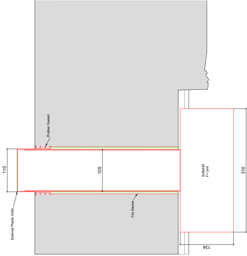
Detail of Sonair Unit Scale: 1:2
