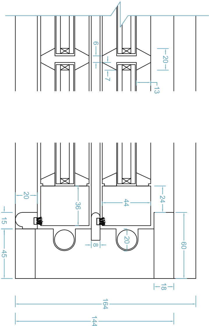
PLAN SECTION scale 1:2
