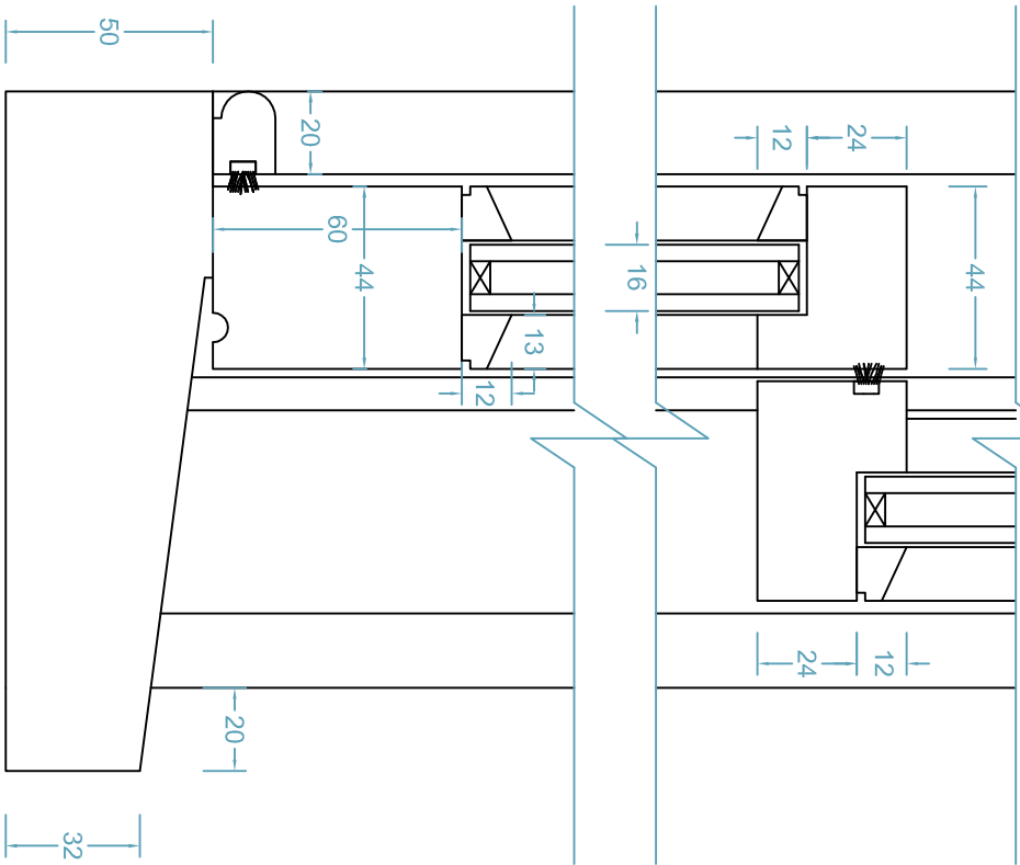
HEIGHT SECTION scale 1:2
