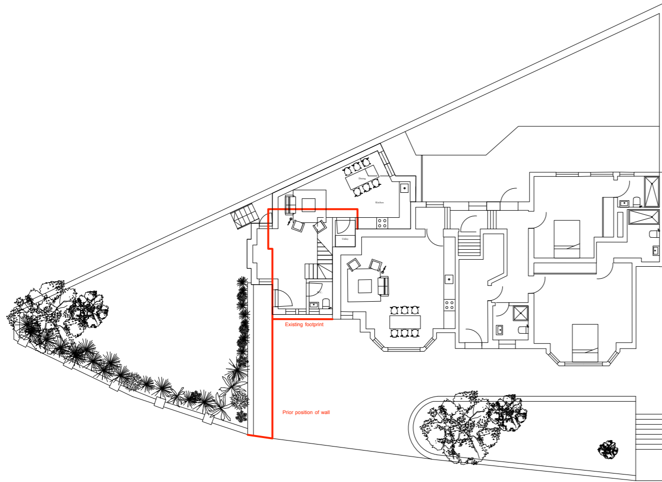
Revised proposal: Ground floor plan 1:200 @ A3
