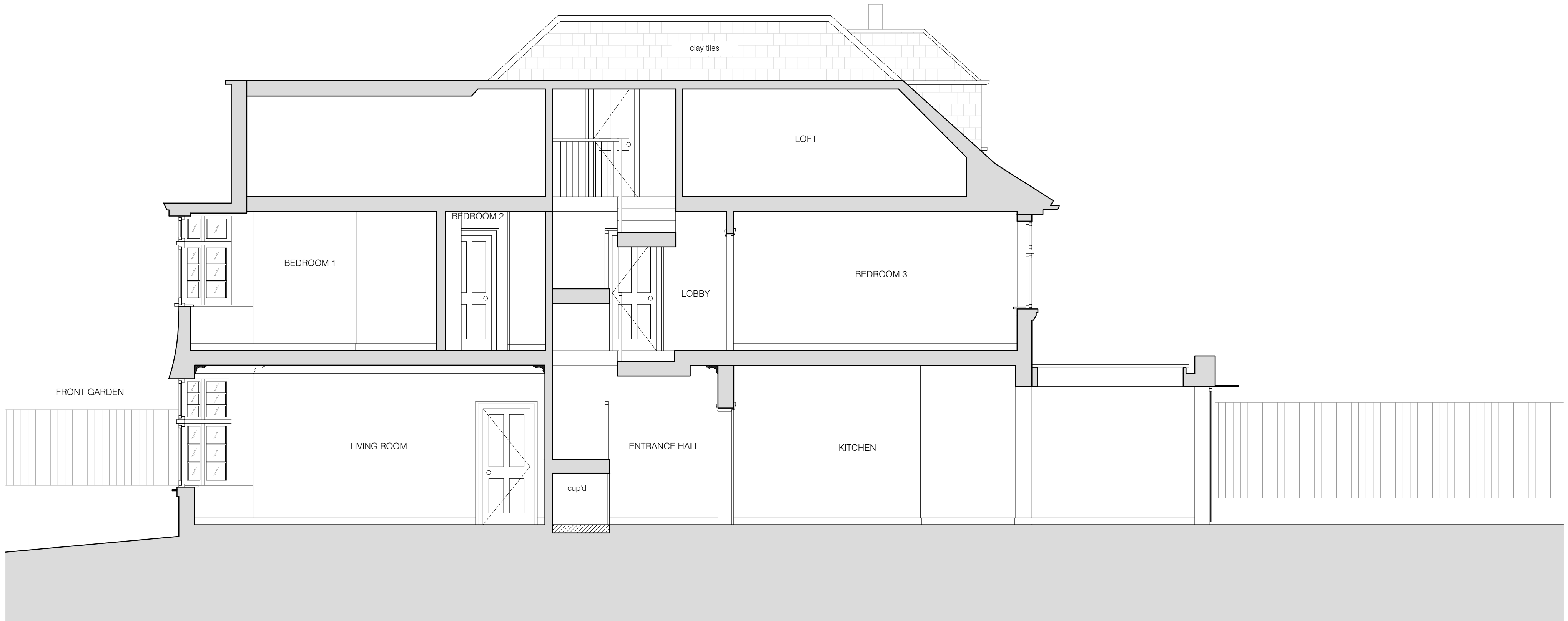
01 EXISTING SECTION A-A scale 1:50
