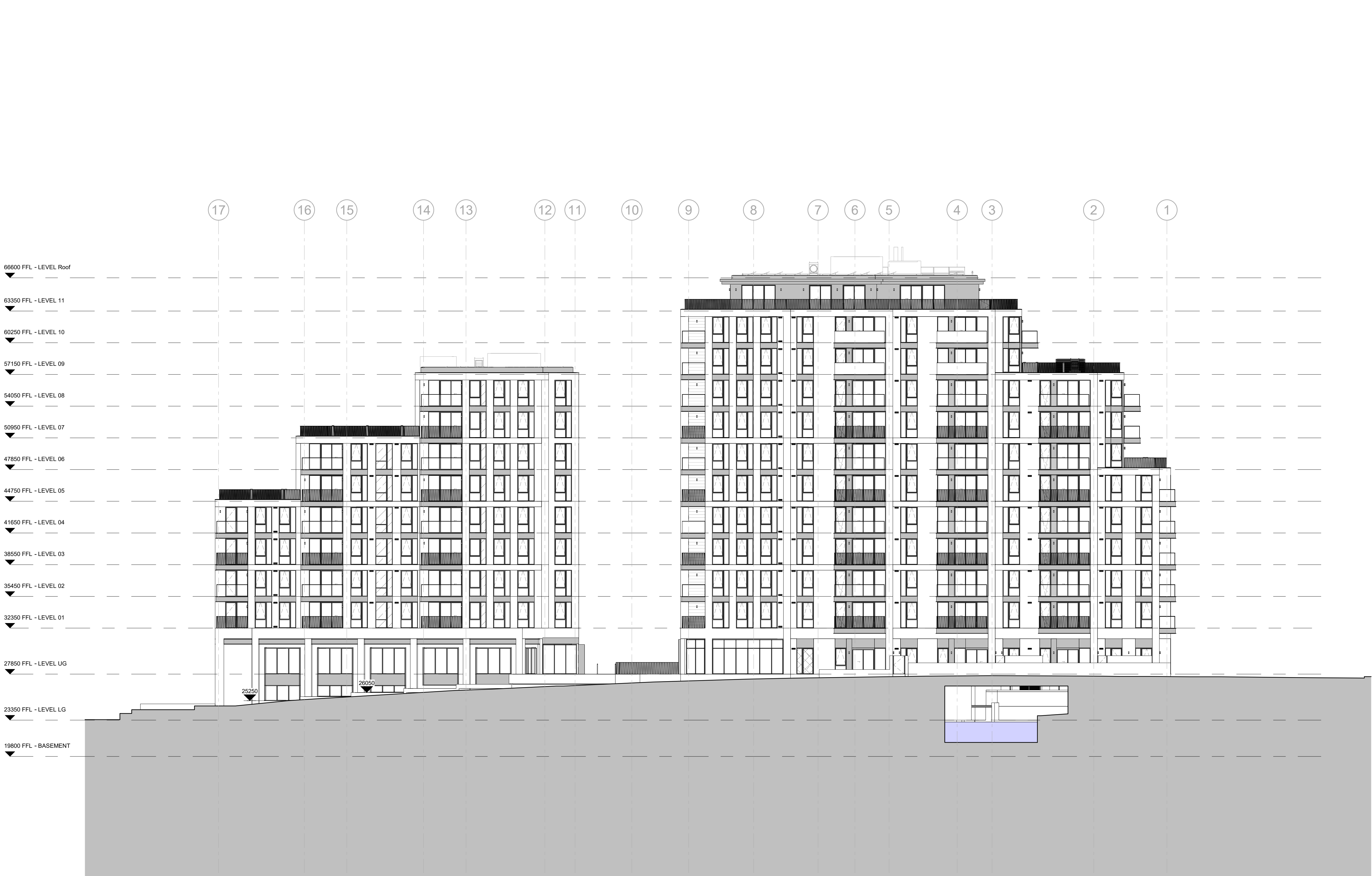
01 - Existing GA NE Elevation
