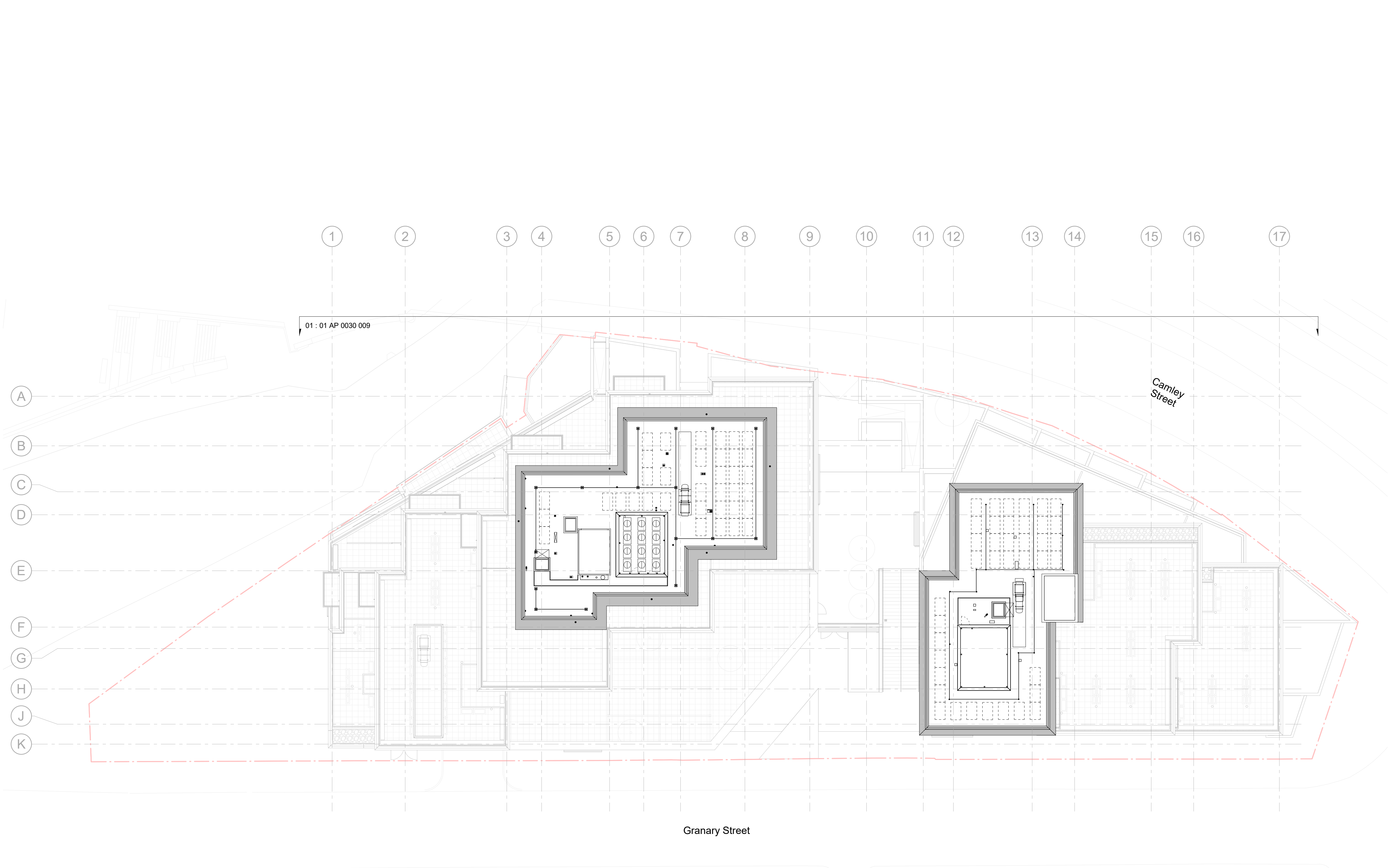
01 - Existing Roof Level Services Layout
