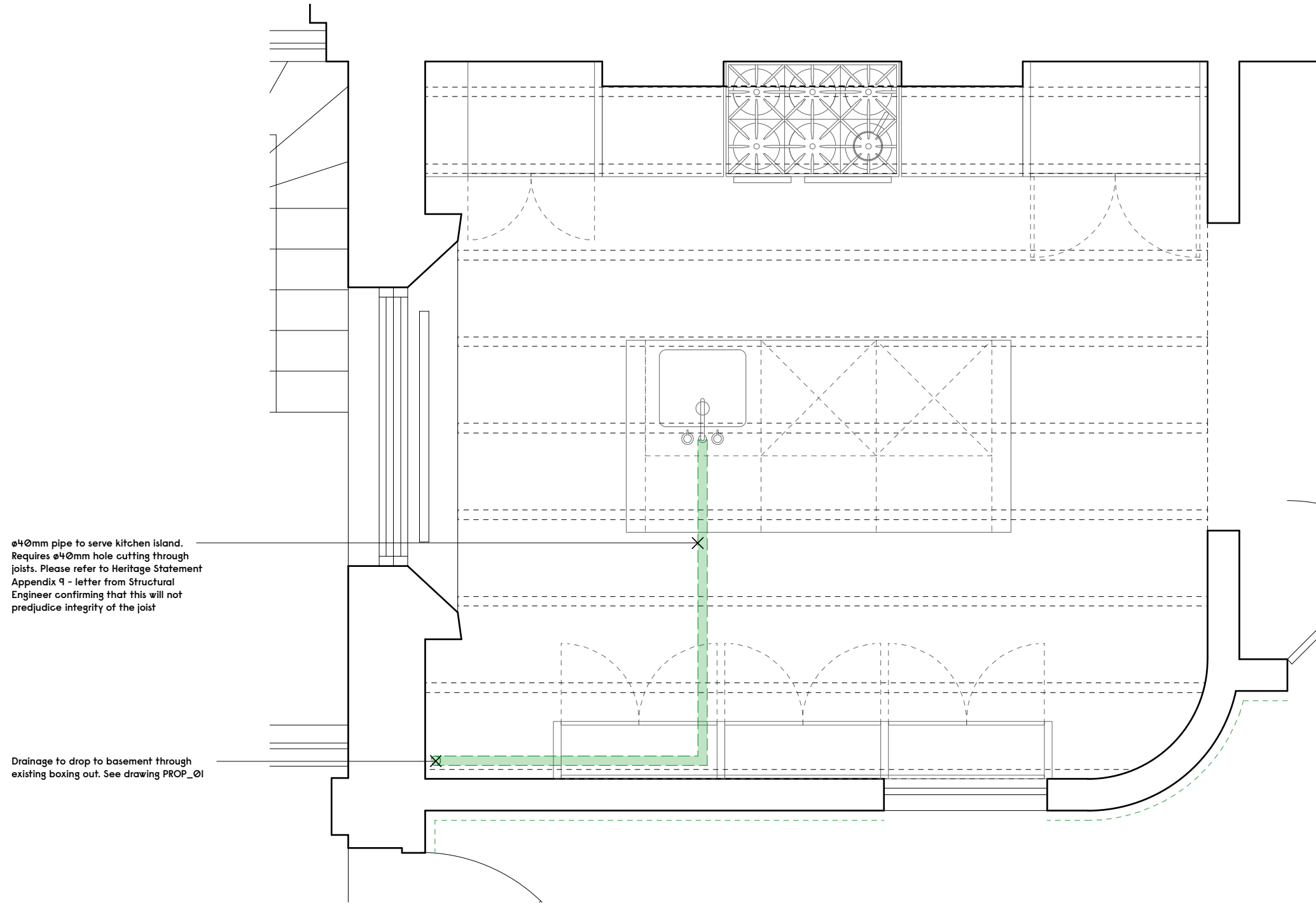
1 Proposed Ground Floor Drainage 1:25 @ A3
