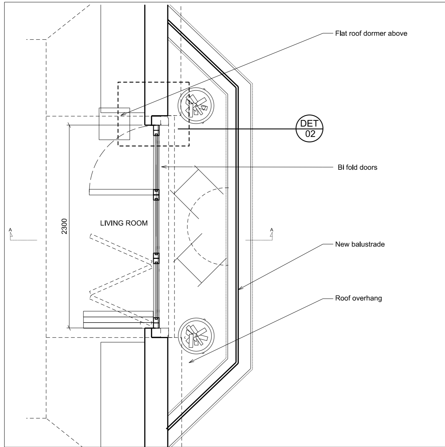
01 DETAIL PLAN 1:25@A3
