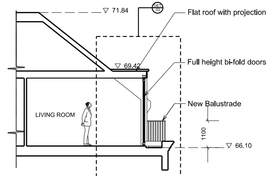
02 PROPOSED SECTION A-A
