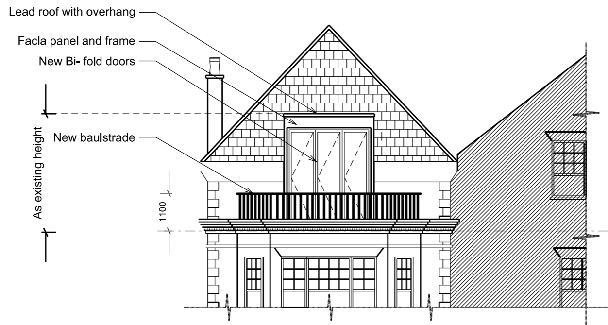
03 PROPOSED REAR ELEVATION
