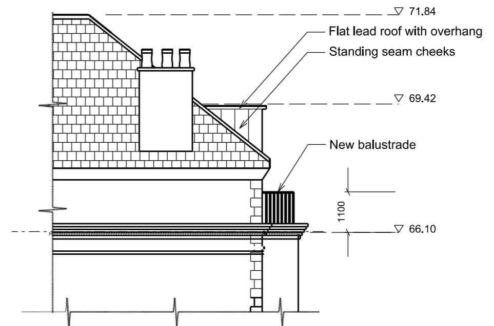
04 PROPOSED SIDE ELEVATION
