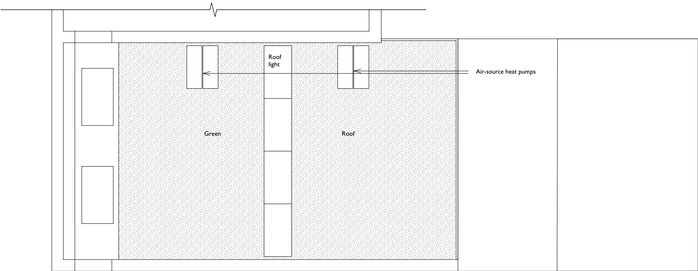
ROOF PLAN
