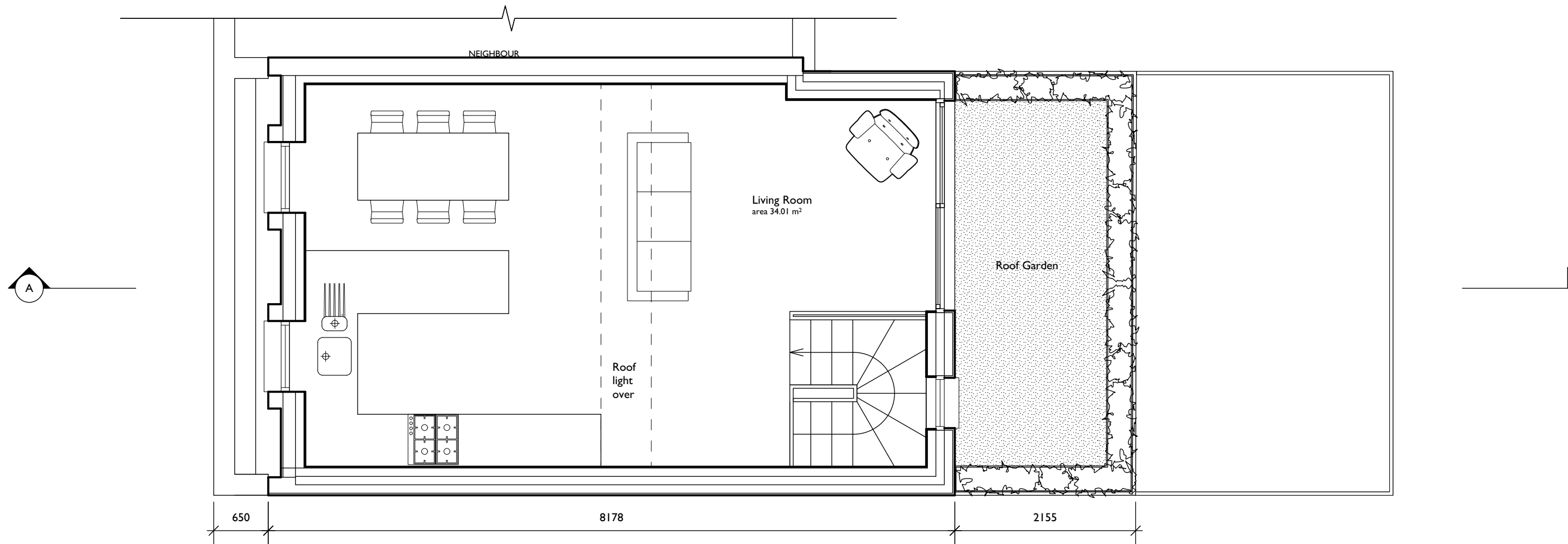
THIRD FLOOR PLAN GIA 34.01 m 2
