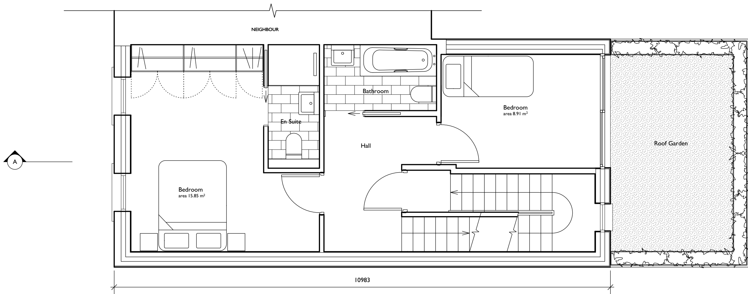
SECOND FLOOR PLAN GIA 40.15 m 2
