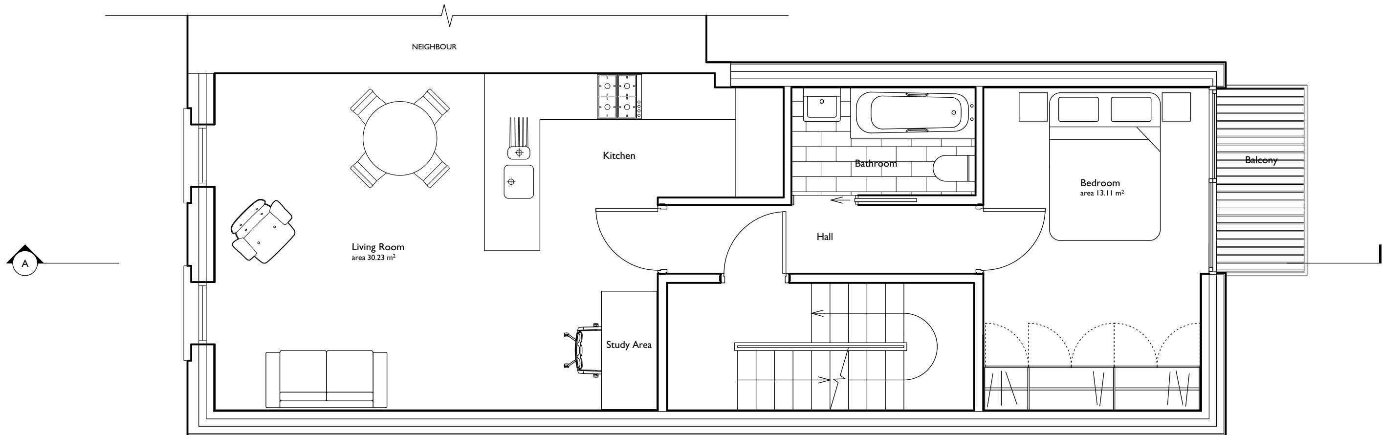
FIRST FLOOR PLAN GIA 51.92 m 2
