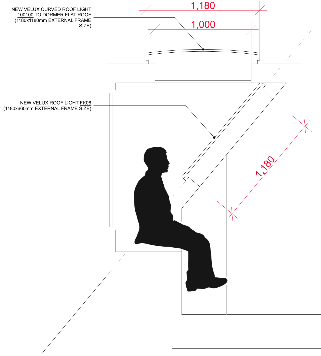
3 VELUX SPECIFICATION
