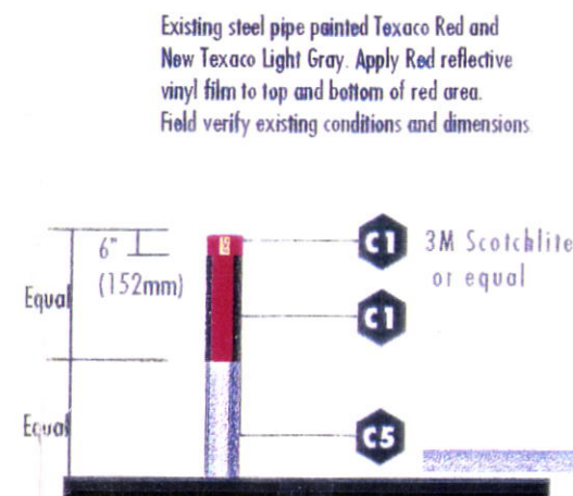
C BOLLARD DETAIL Scale: 3/16" = 1' - 0"
