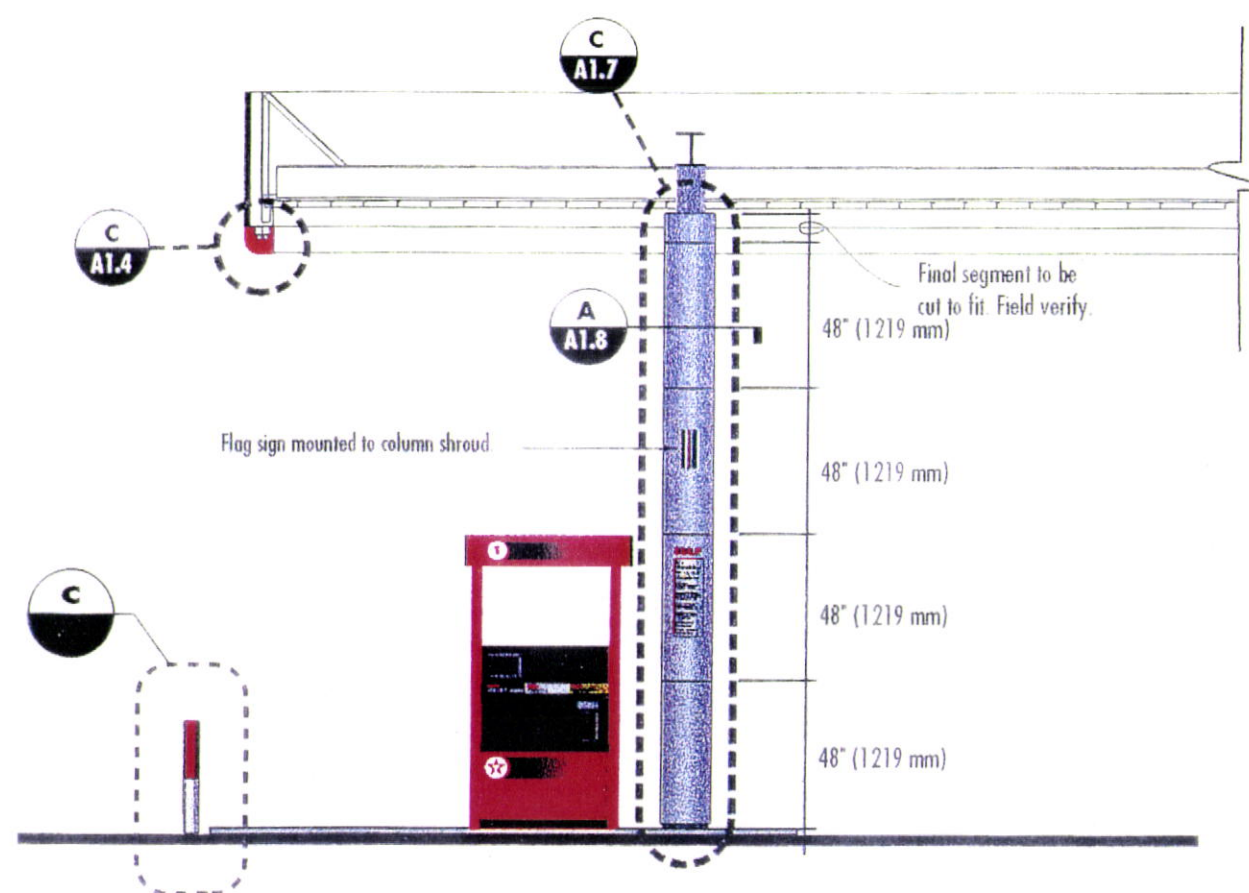
A PARTIAL CROSS SECTION - Thru Canopy Scale: None
