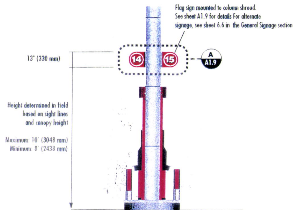
B End View - Gas Island Scale: None
