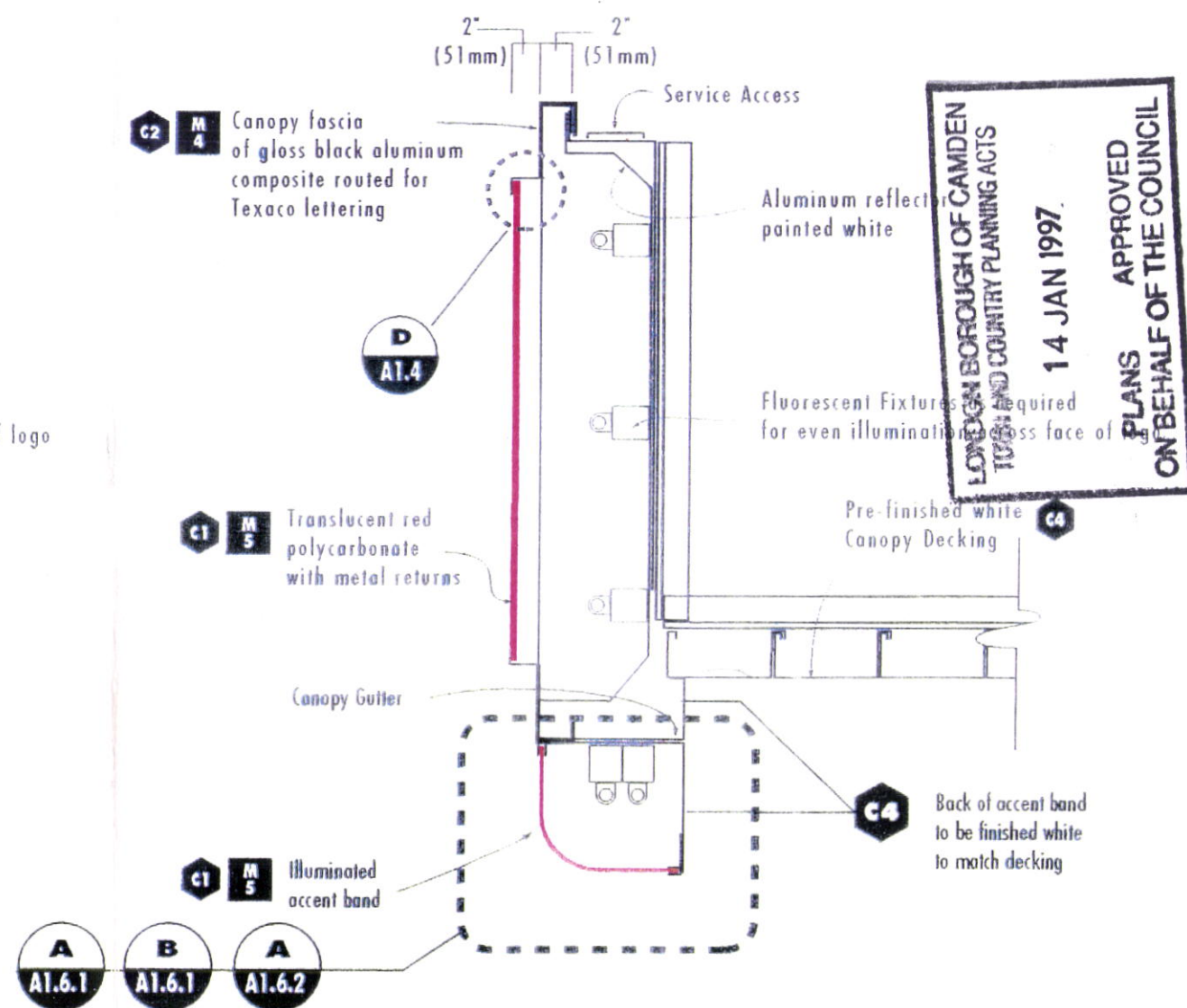
B SECTION at Logotype (If new signage is required) Scale: None
