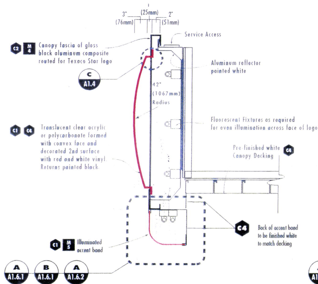
A SECTION at Star Logo (If new signage is required) Scale: None
