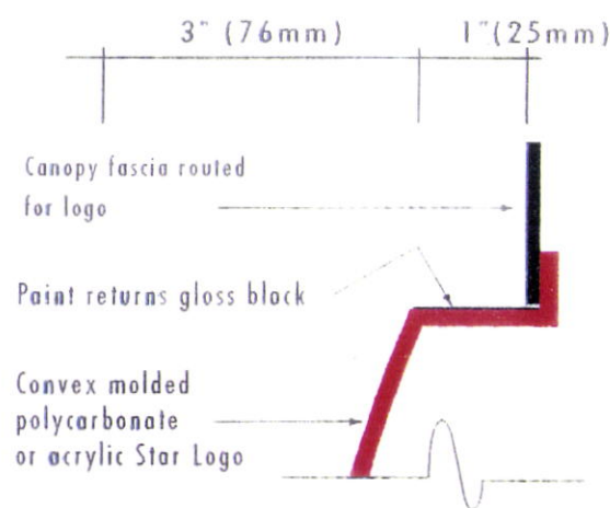
A SECTION at Star Logo (If new signage is required) Scale: None
