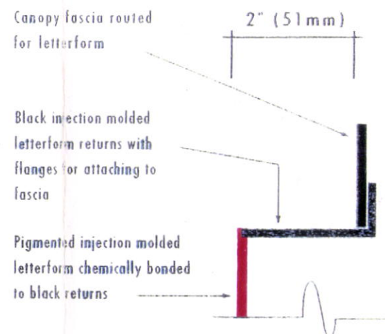
D DETAIL SECTION at Logotype Scale: None
