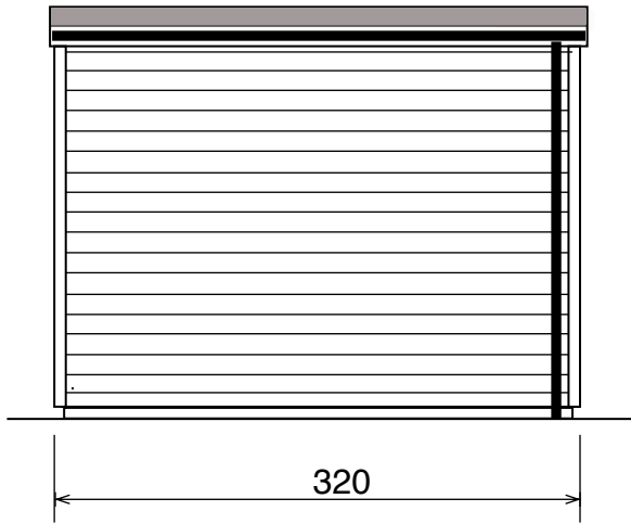
Back elevation
