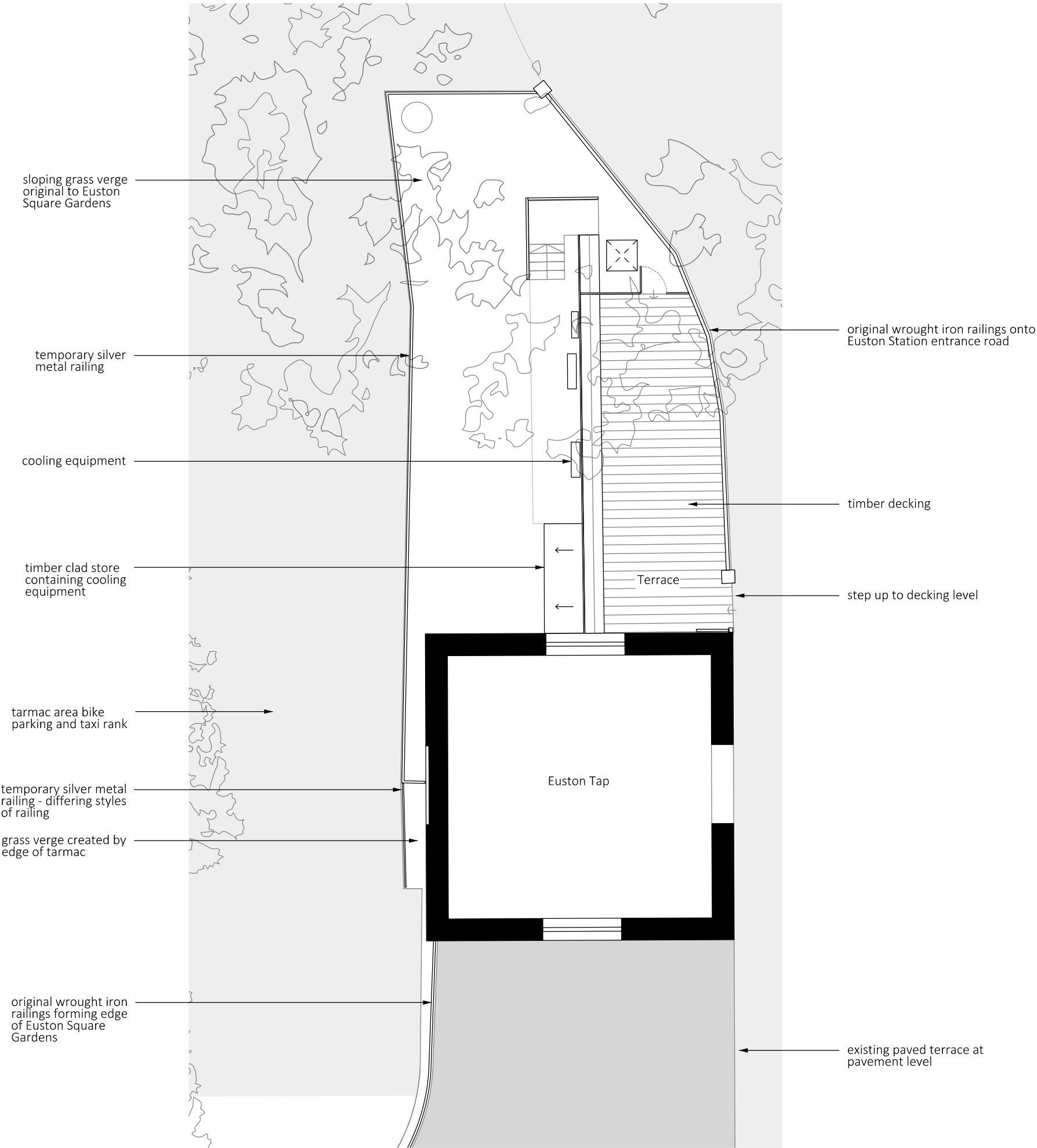
01 Existing Ground Floor Plan
