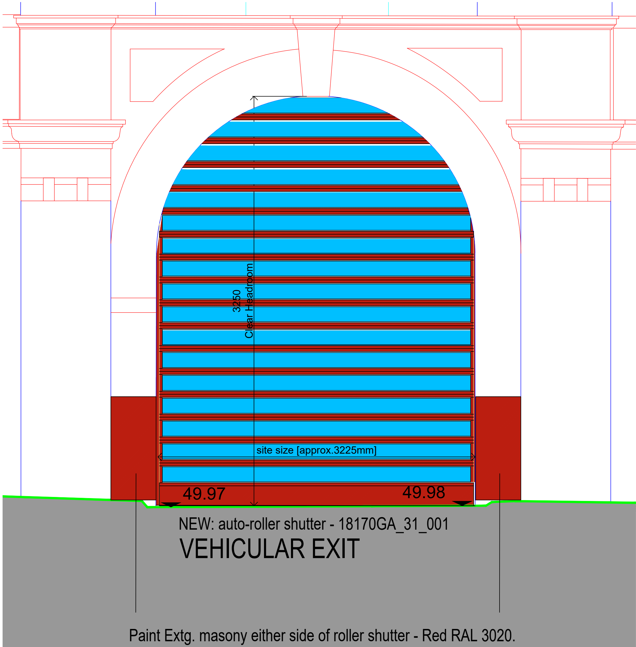
Fast Response Shutter ELEVATION: Scale; nts.
