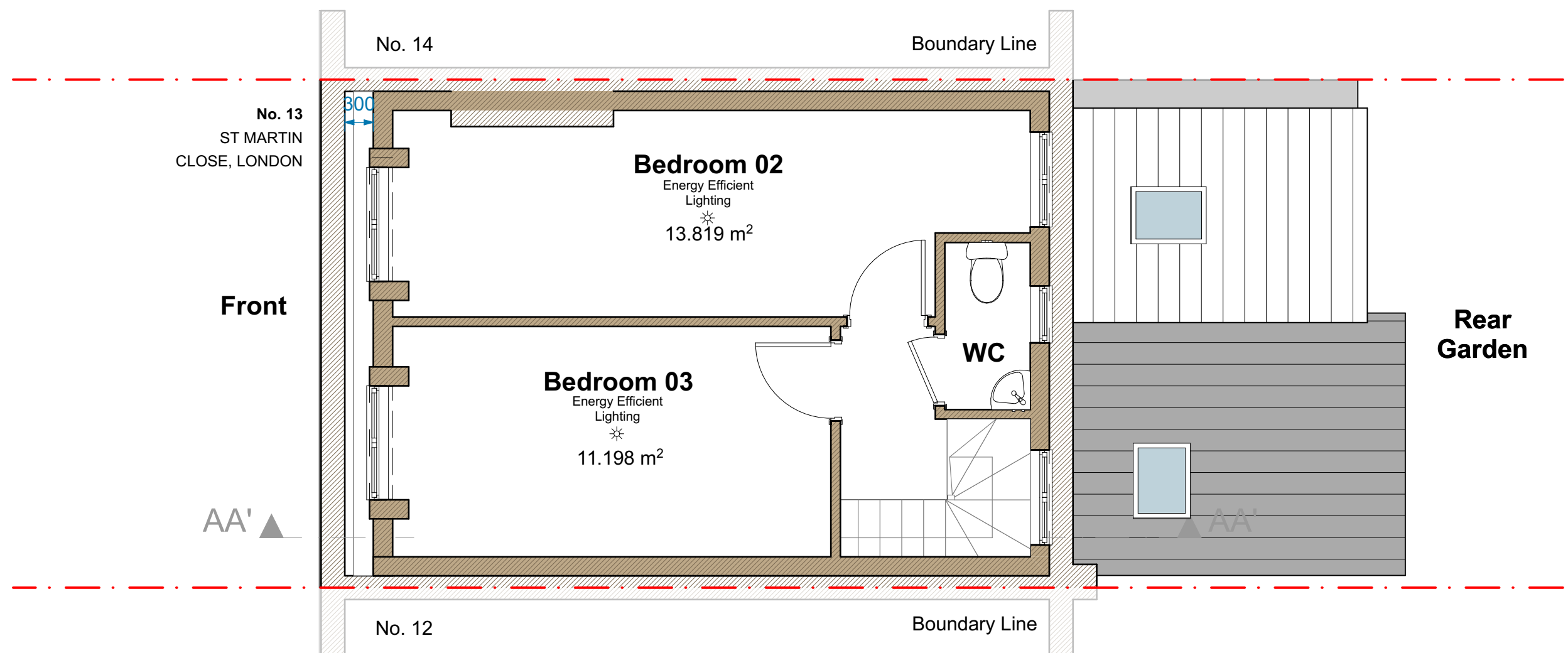
Proposed Third Floor Plan 1:50
