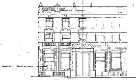
1/100 ELEVATION TO HAMPSHIRE HIGH STREET SHOWING LOCATION OF PROPOSED BARCLAY BANK
