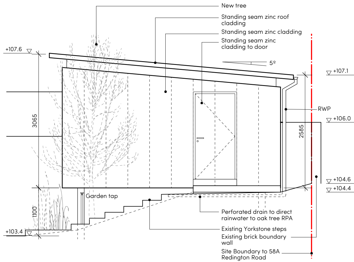
A PROPOSED NORTH EAST ELEVATION 1:50 @ A3
