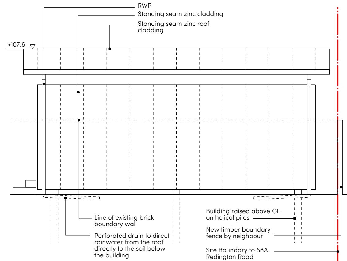
A PROPOSED NORTH EAST ELEVATION 1:50 @ A3
