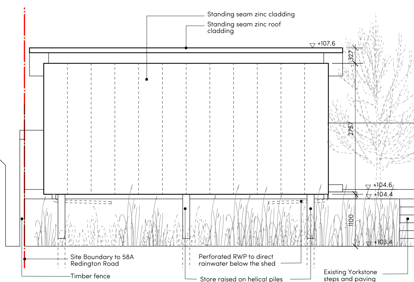
D PROPOSED SOUTH EAST ELEVATION 1:50 @ A3
