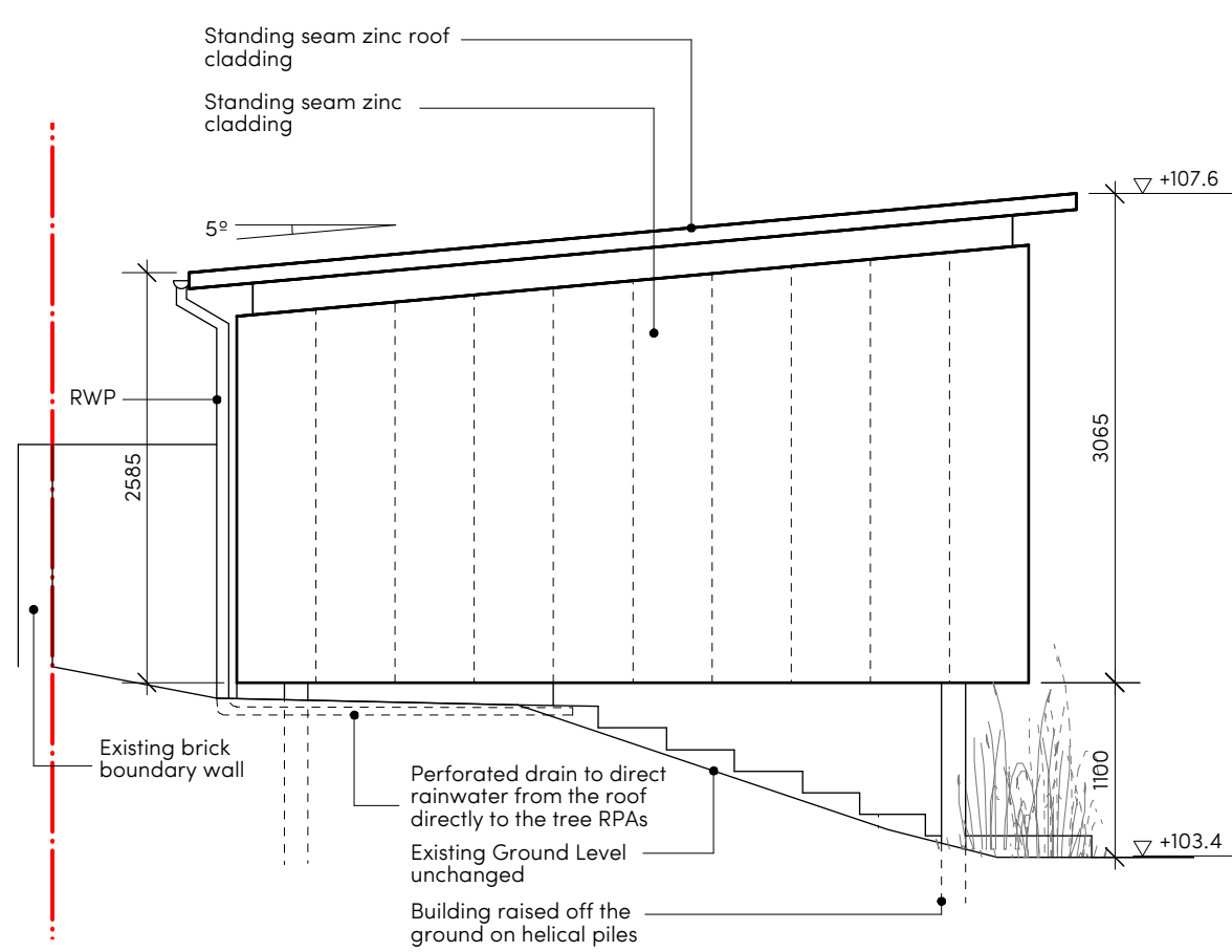
B PROPOSED SOUTH WEST ELEVATION 1:50 @ A3
