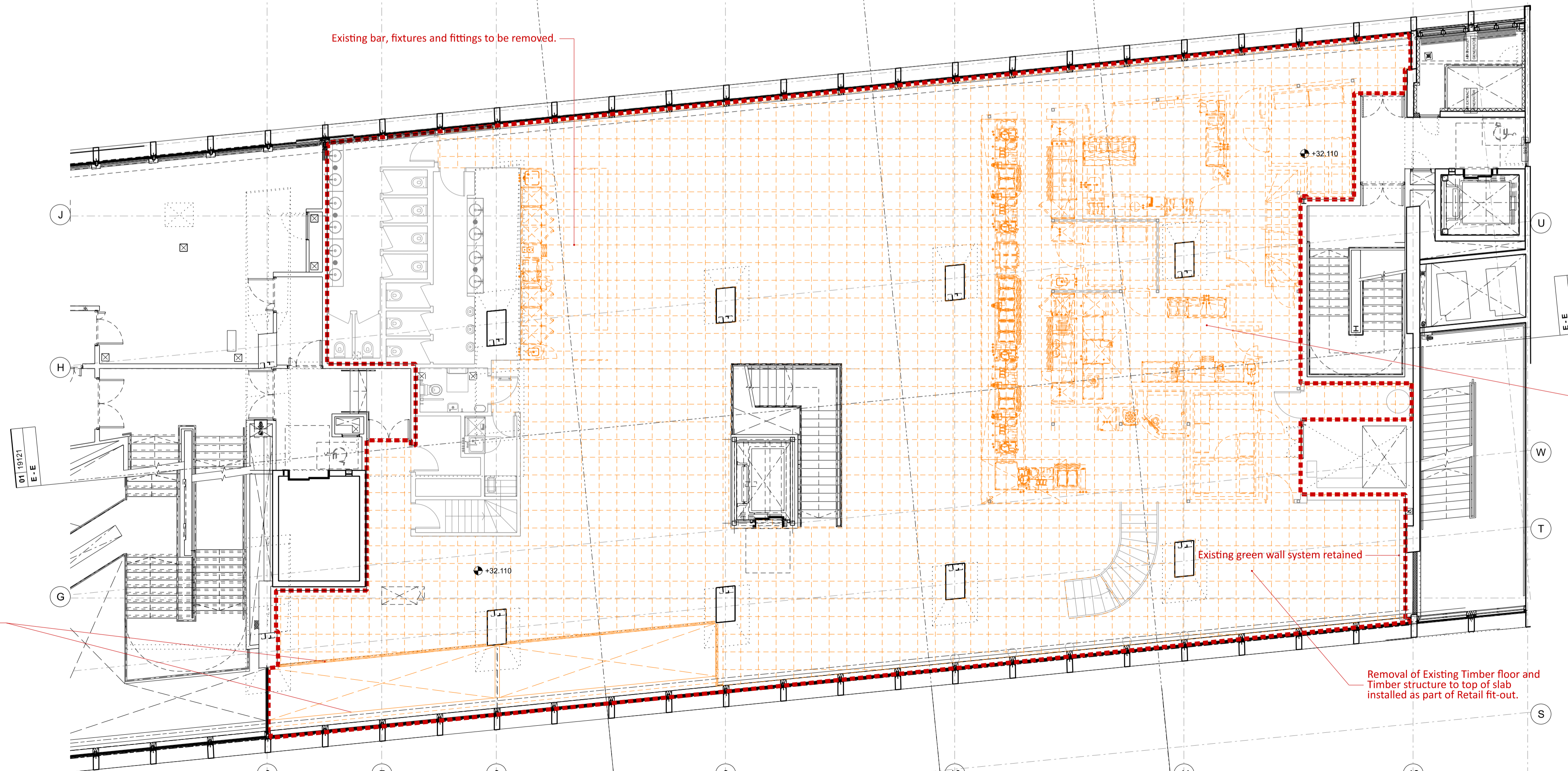
First Floor plan 709-19111
