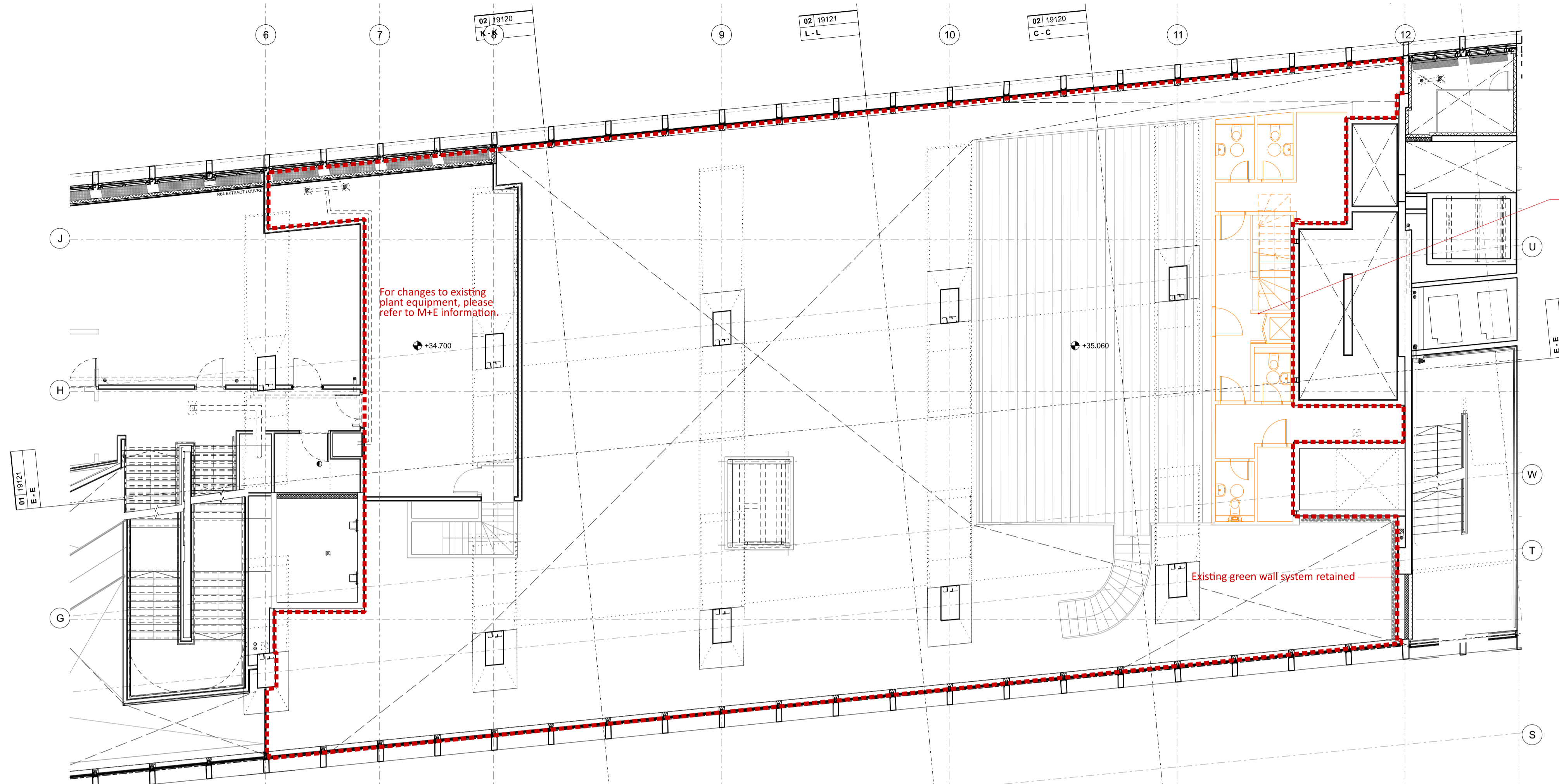
First Floor Mezzanine plan 709-19111
