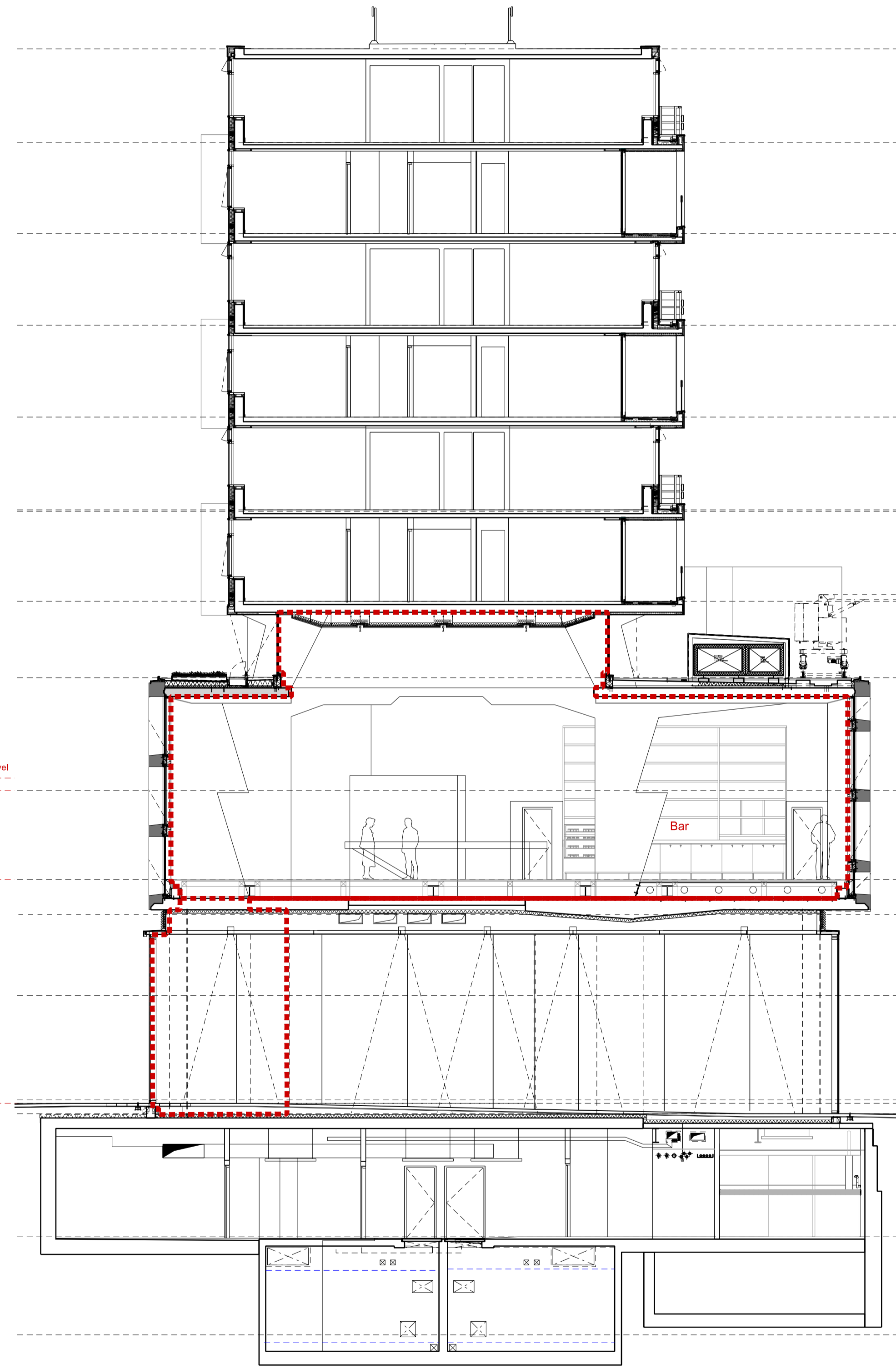
Section LL 709-19021 Centre Point House Earnshaw Street
