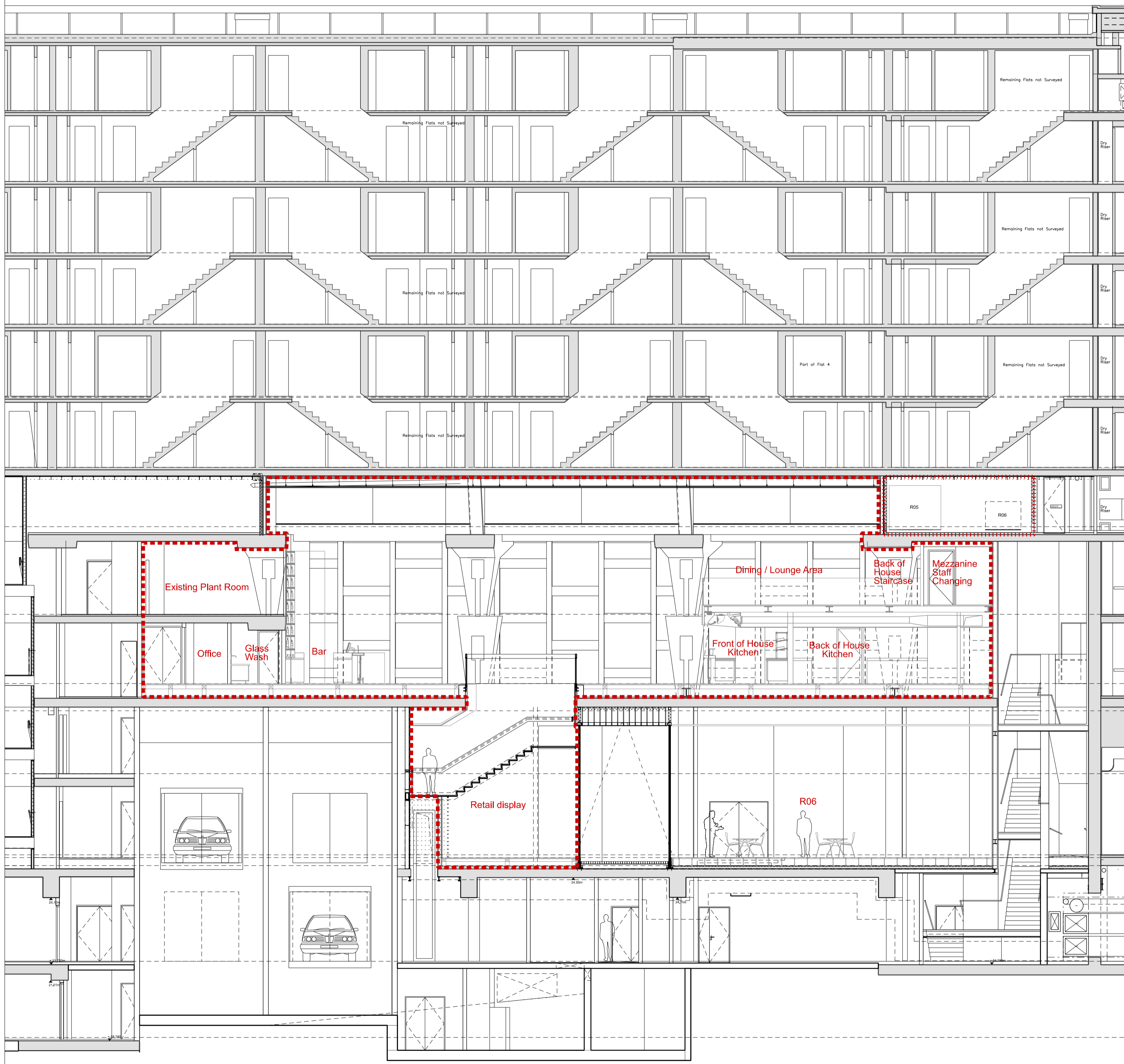
Section EE 709-19021 Centre Point House White Lion House →
