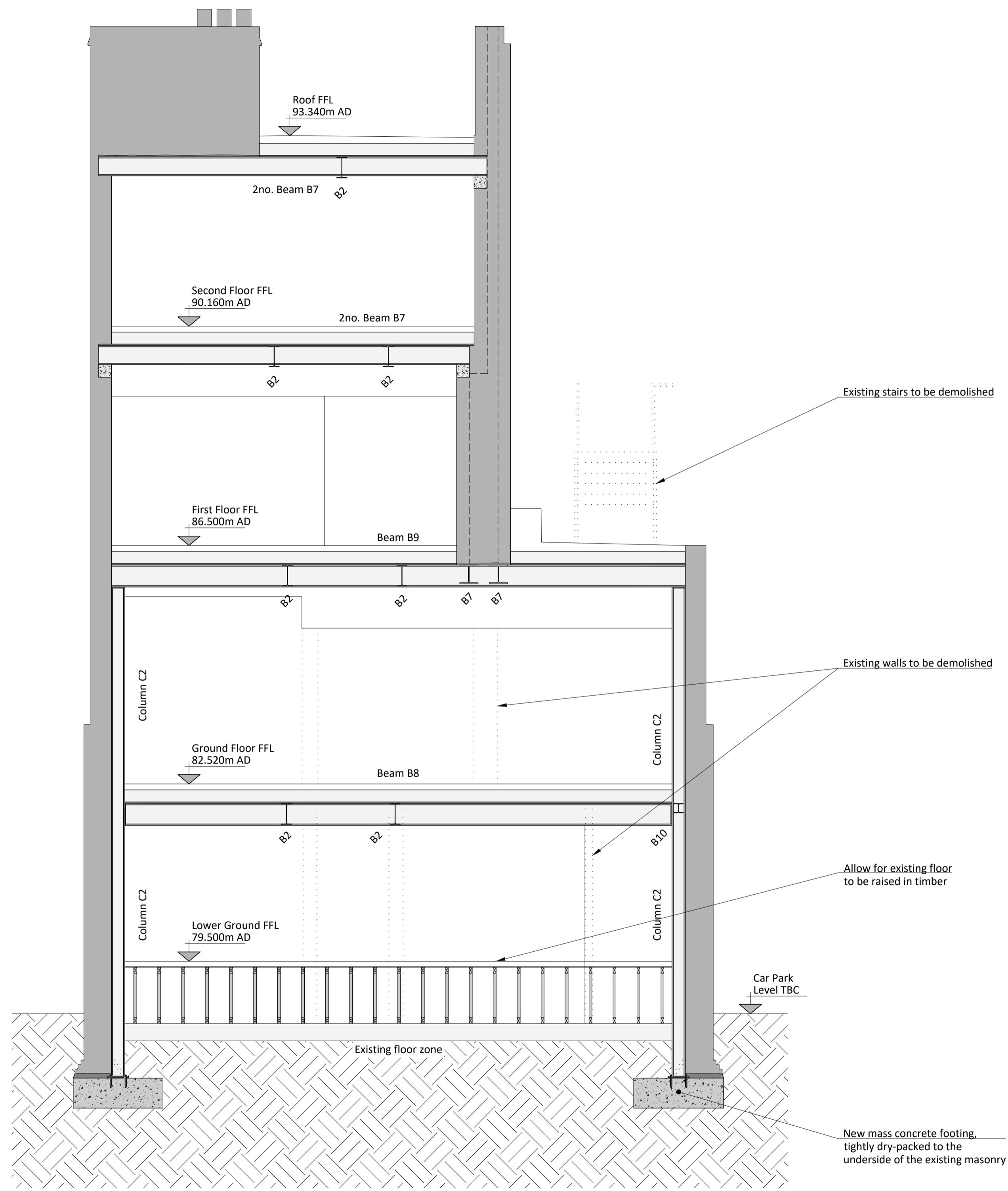
Section A Scale 1:50
