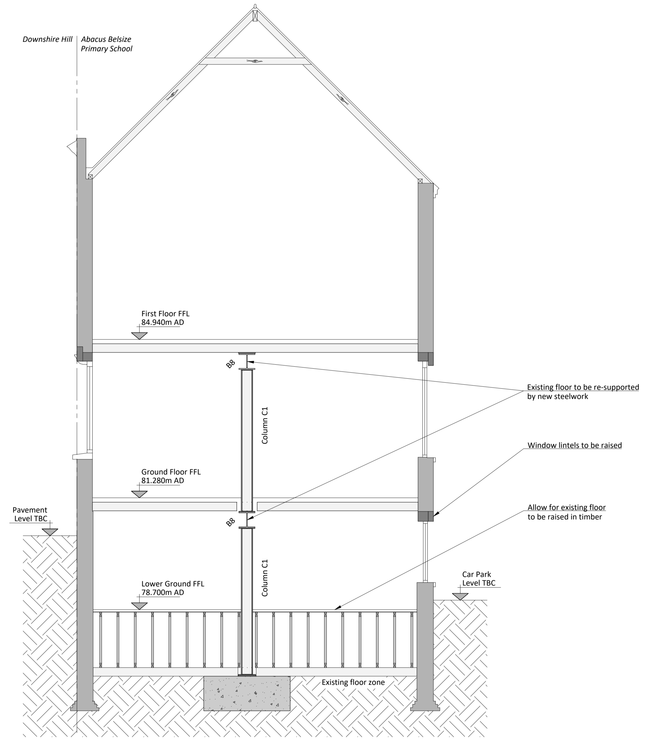
Section B Scale 1:50
