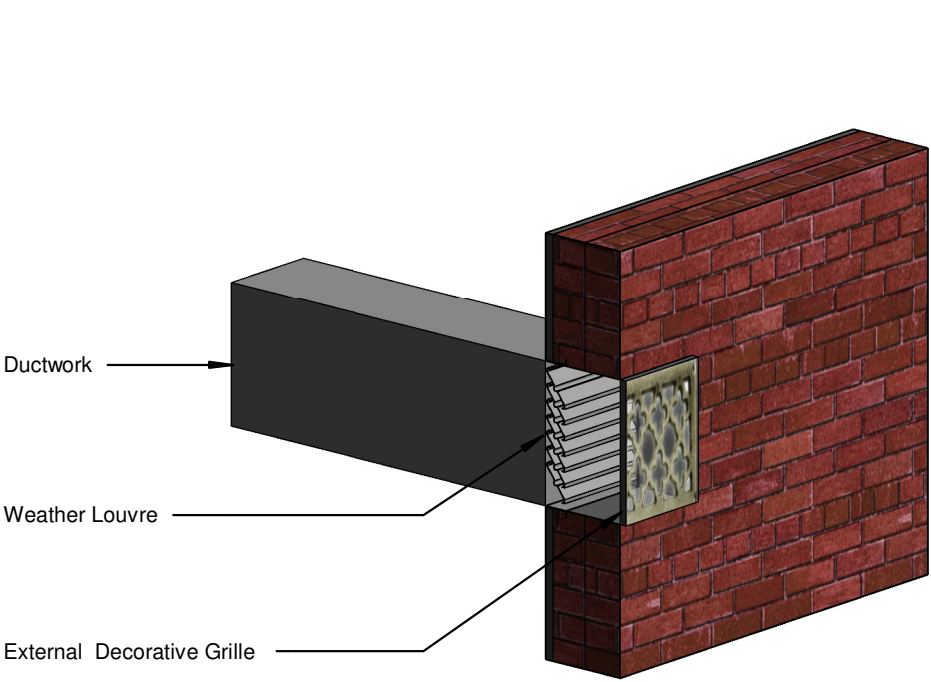
2 3D section
