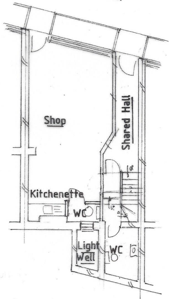
Pre Existing Ground Floor Plan
