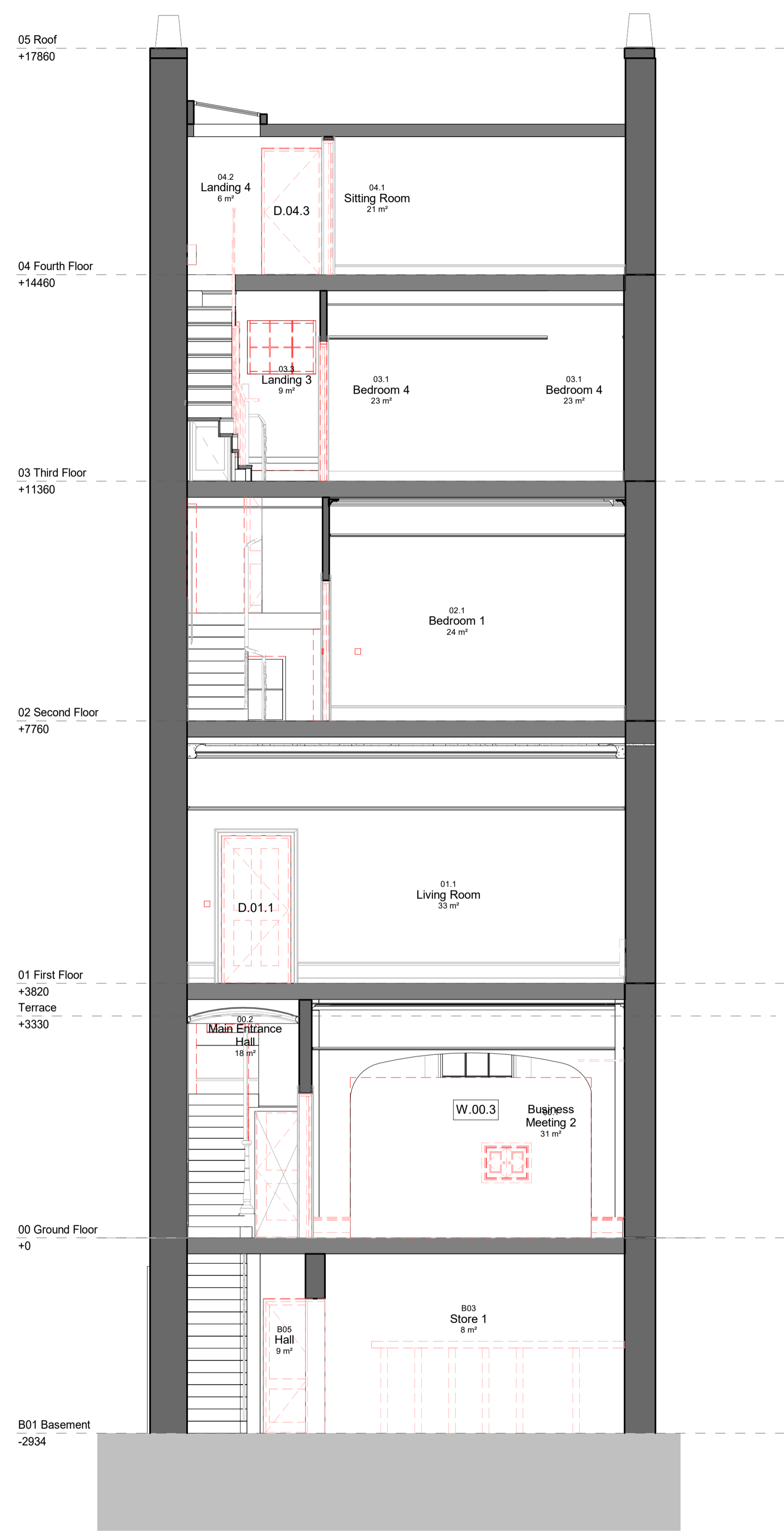
Section C Demolition Scale 1 : 50
