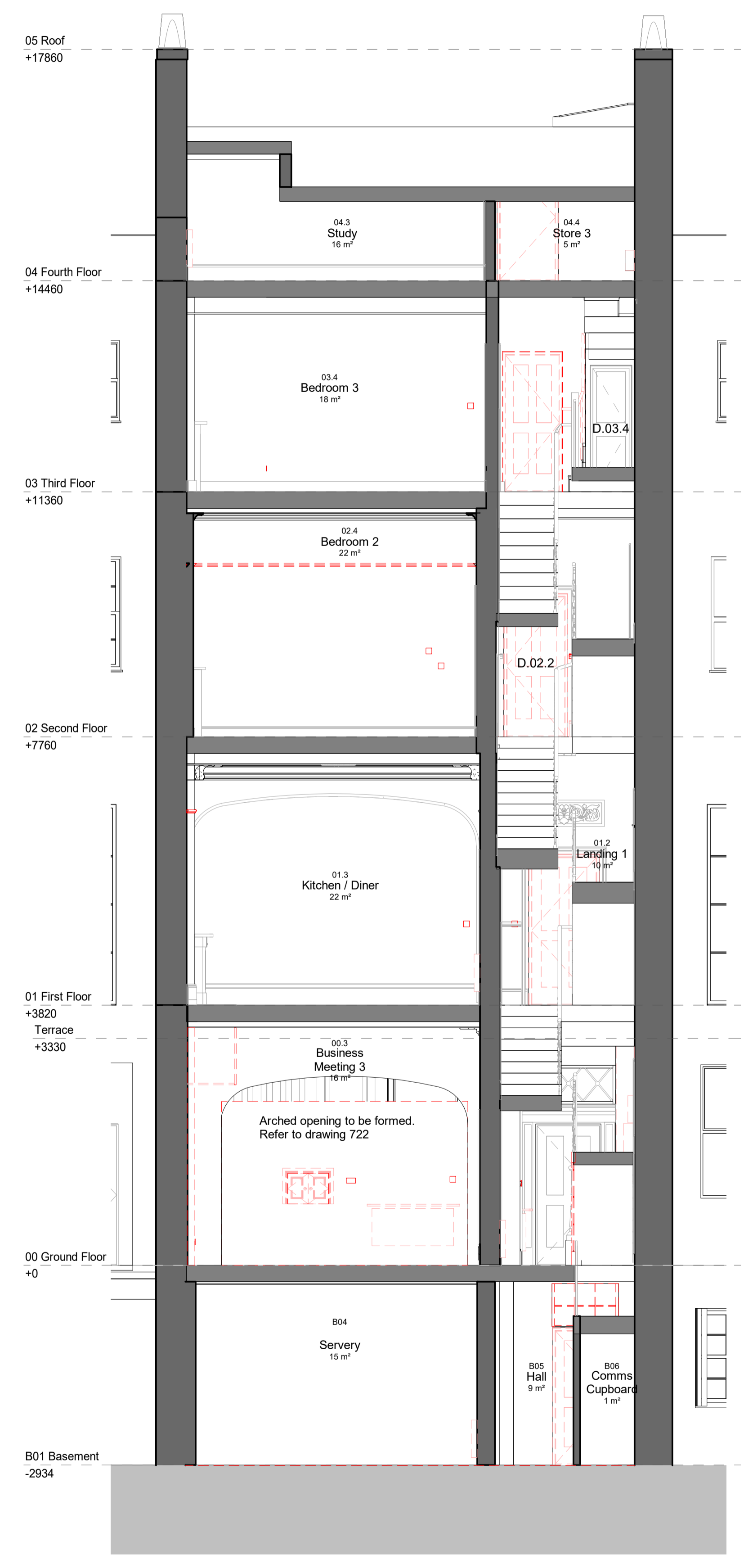
Section D Demolition Scale 1 : 50
