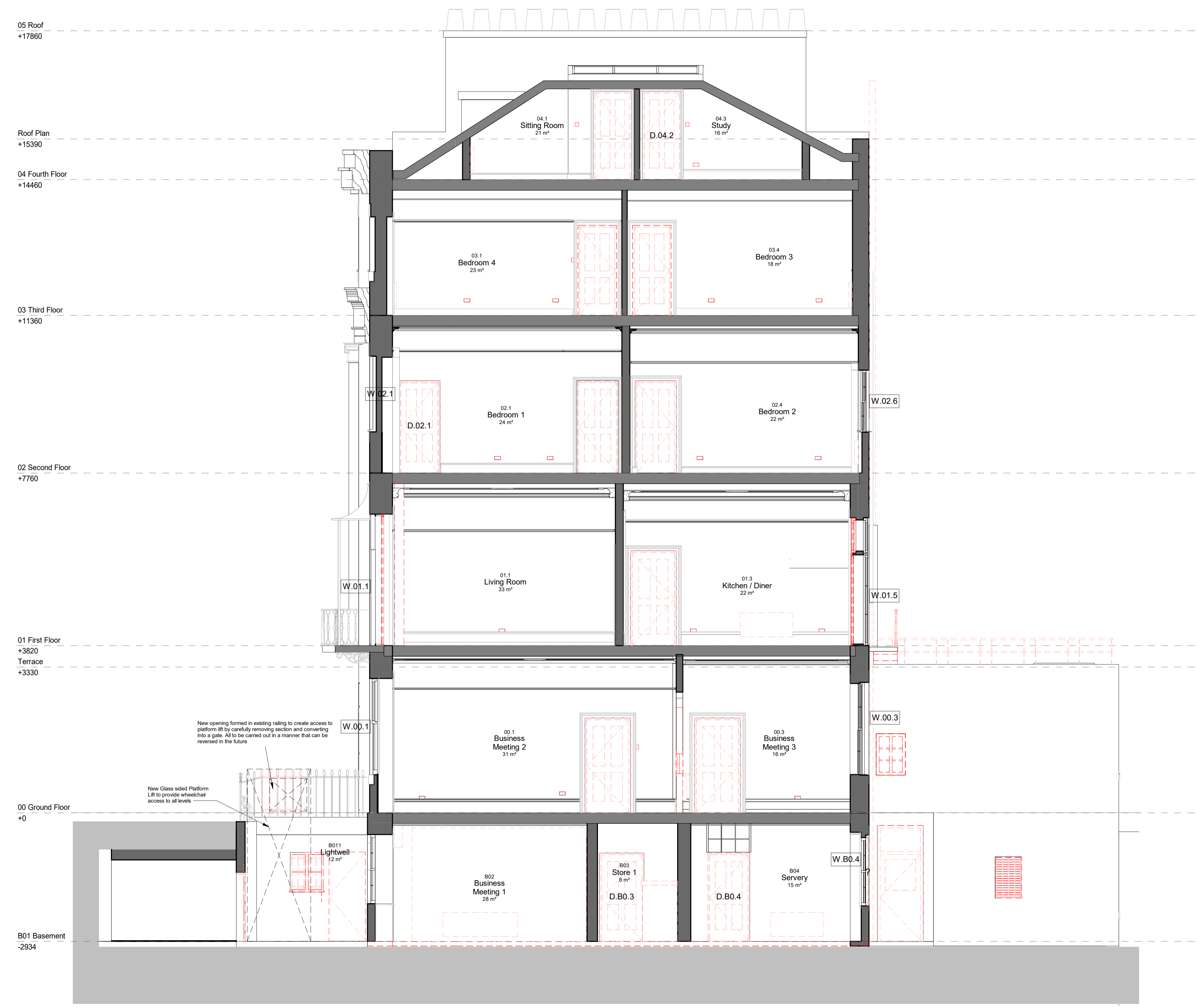
Section B Demolition Scale 1 : 50
