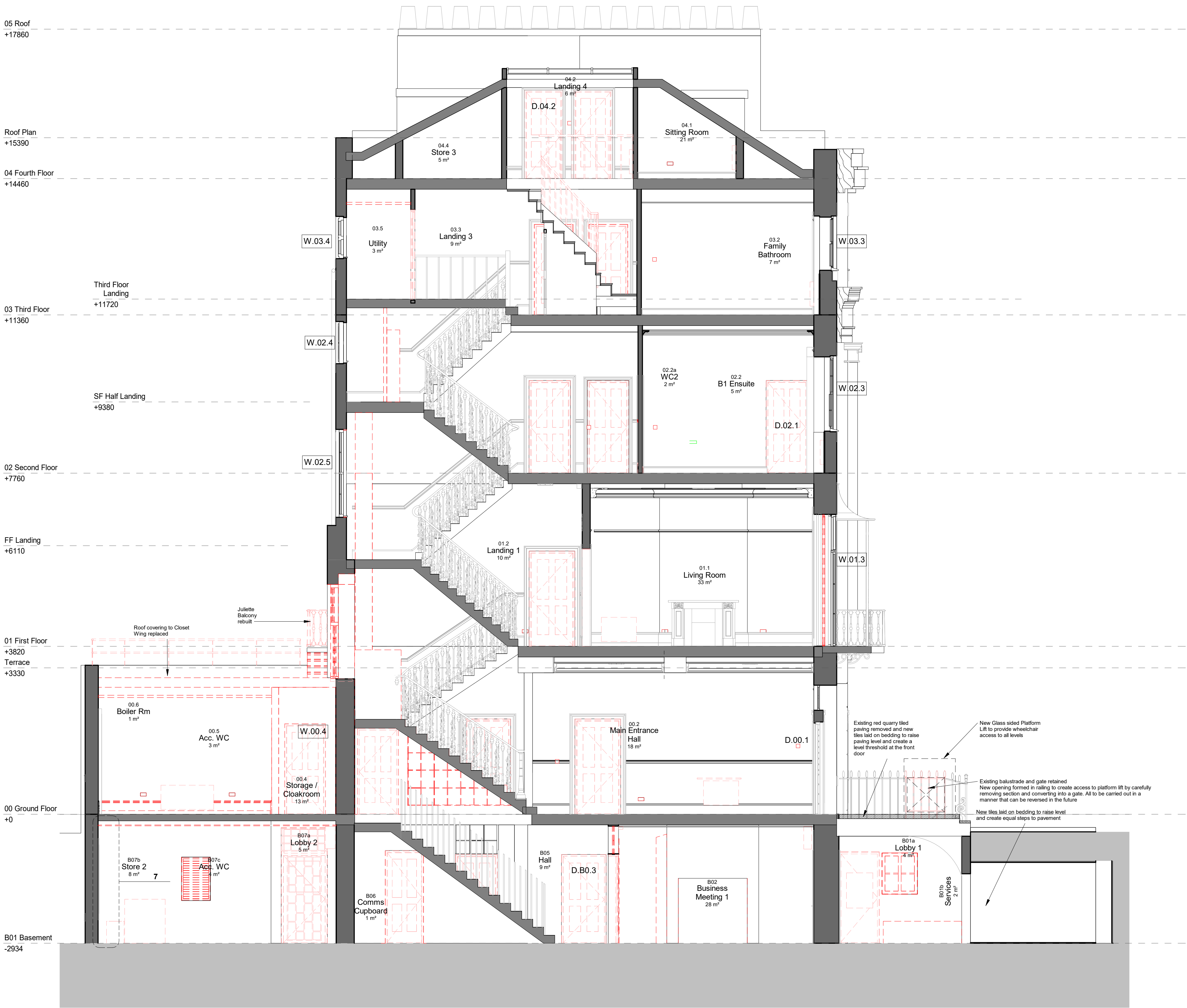
Section A Demolition Scale 1 : 50
