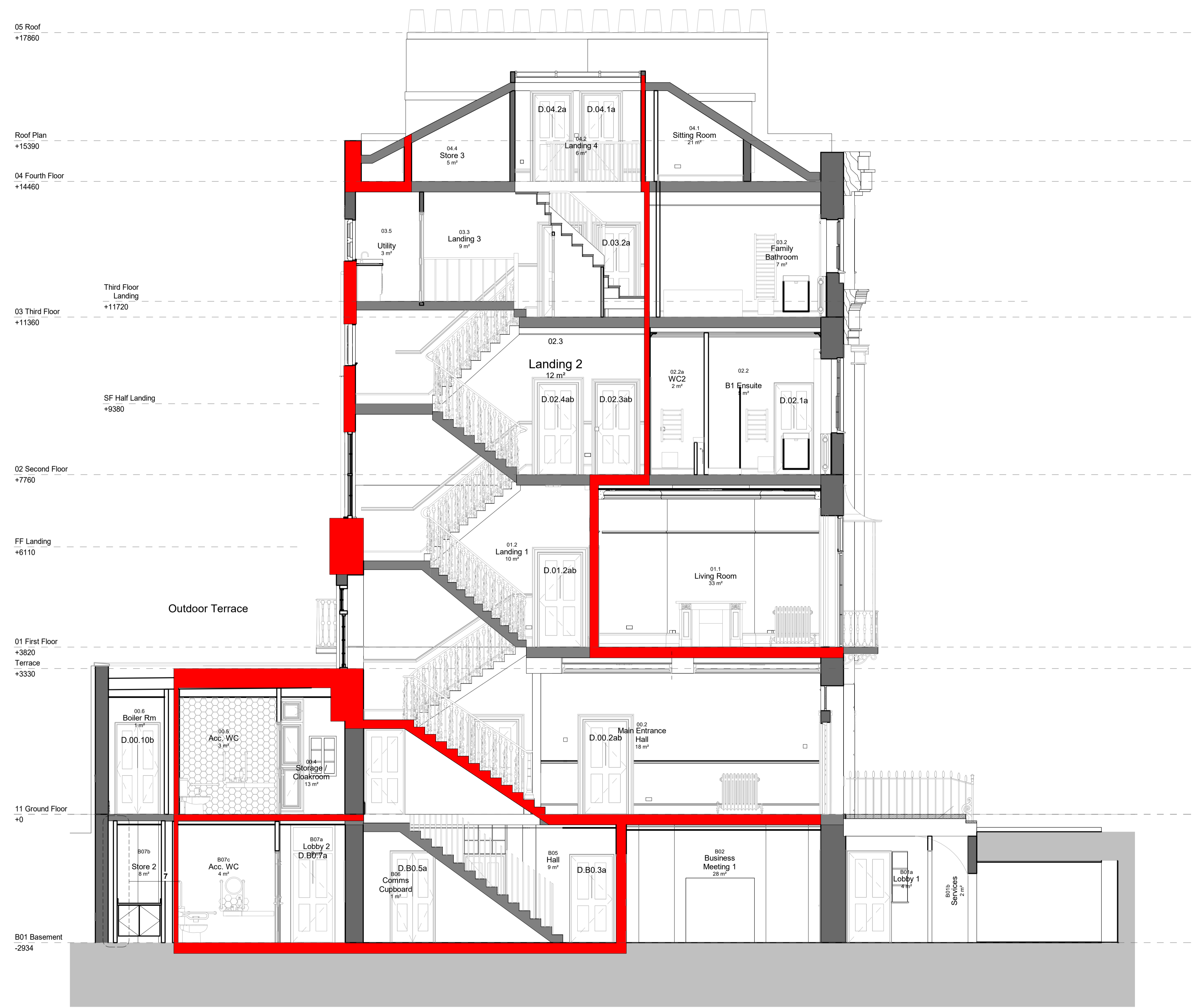
Section F Fire Strategy Scale 1 : 50
