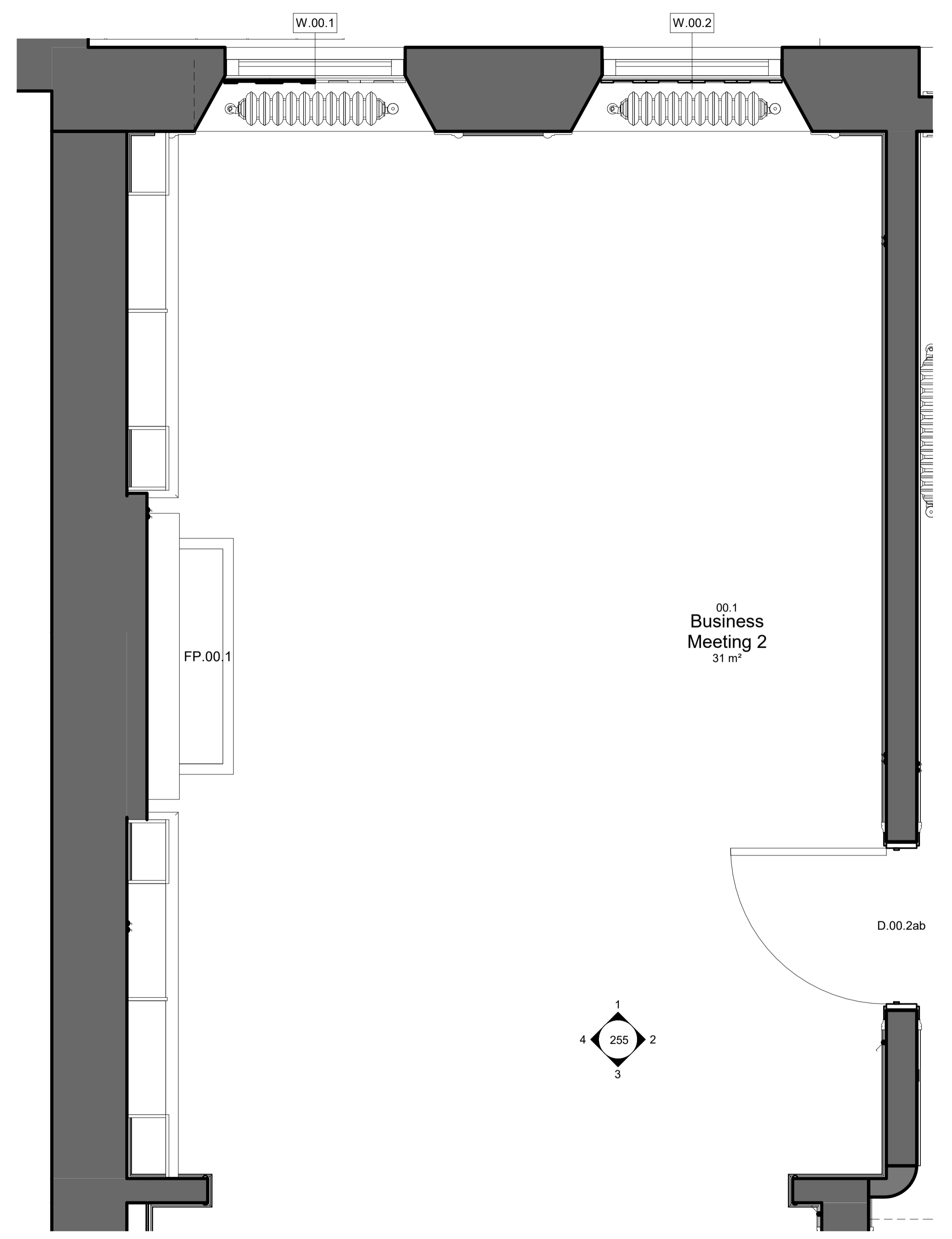
00.1 Business Meeting 2 - Proposed Room Plan Scale 1 : 20
