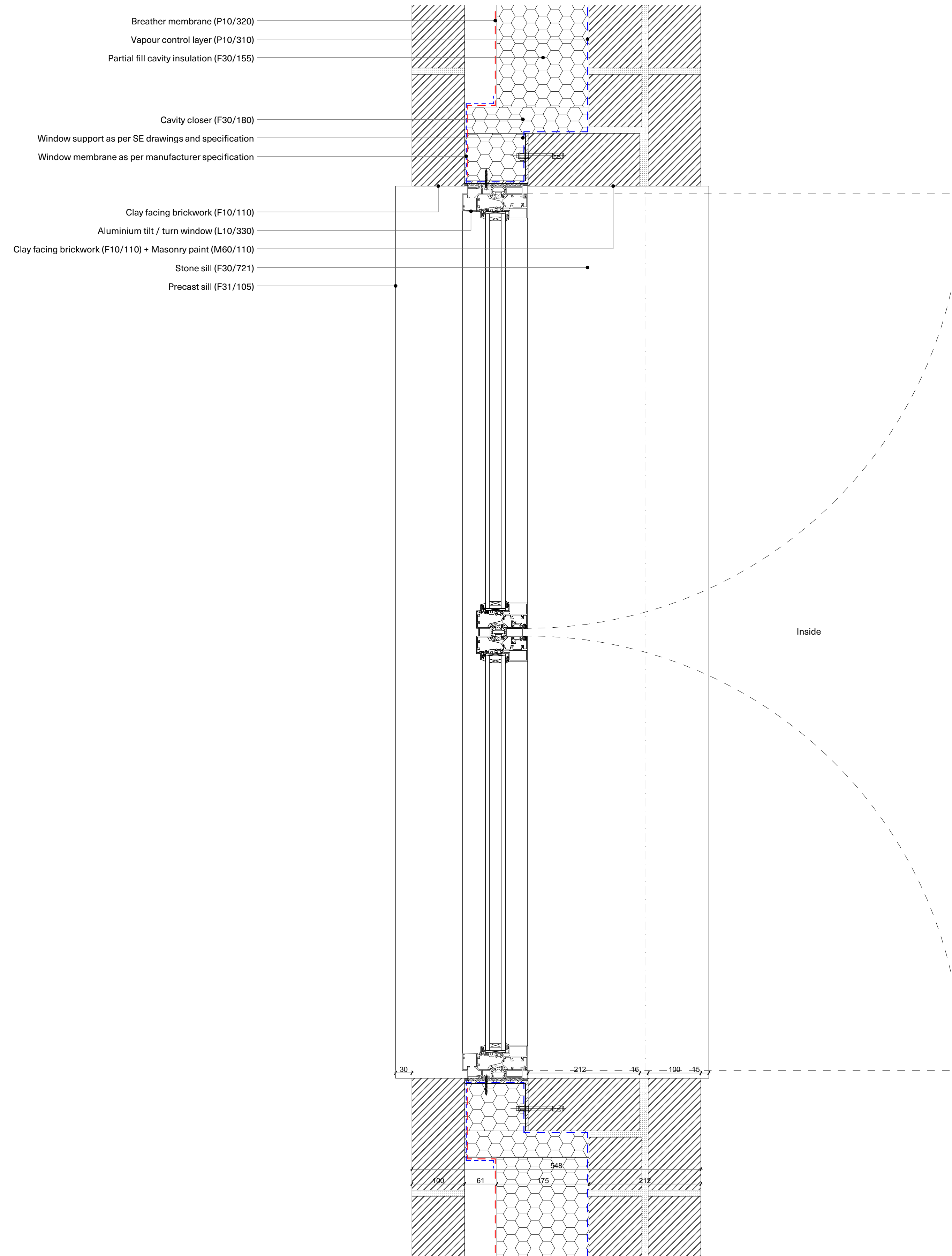
02 Window Jamb Plan Detail
