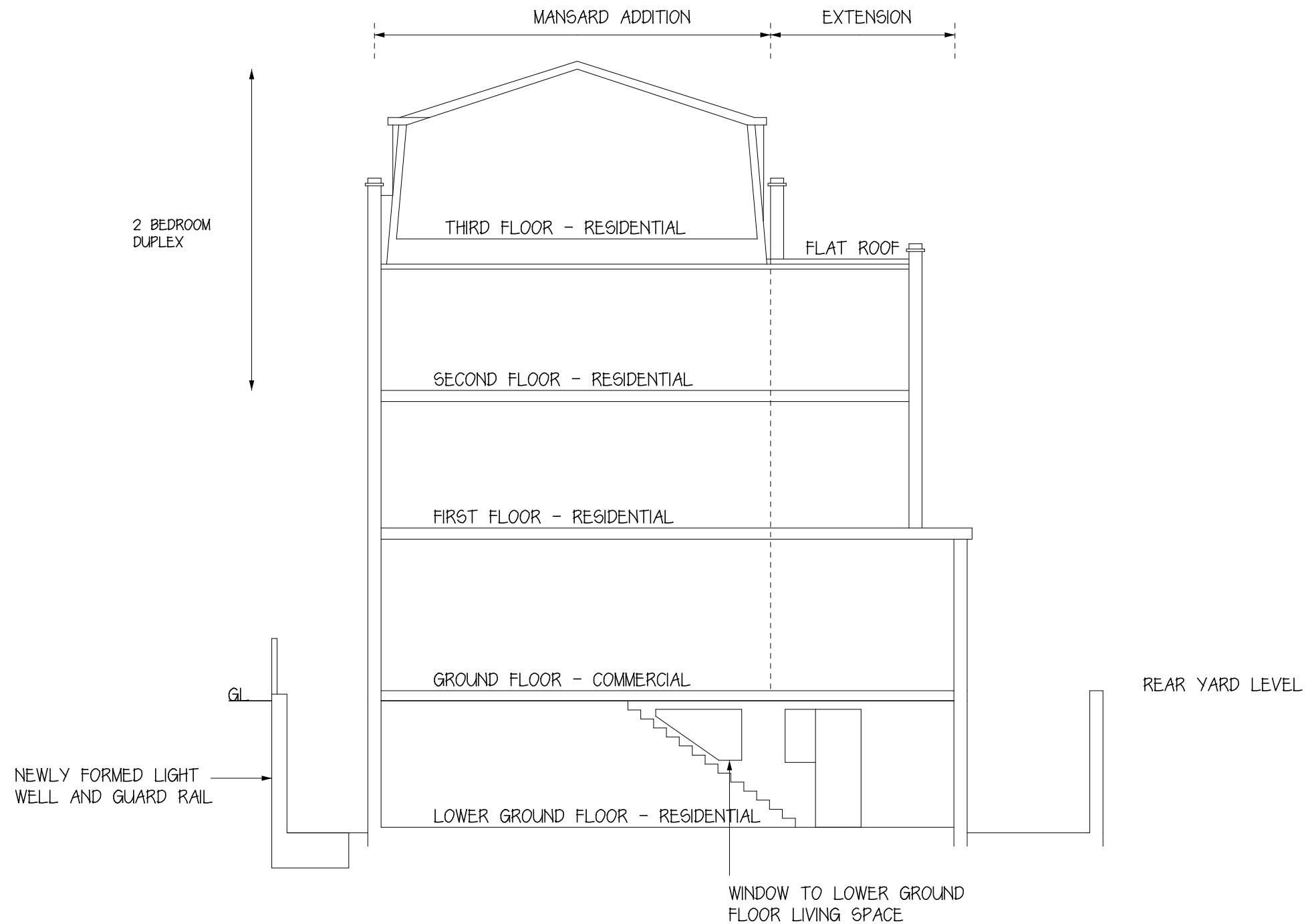
PROPOSED SECTION
