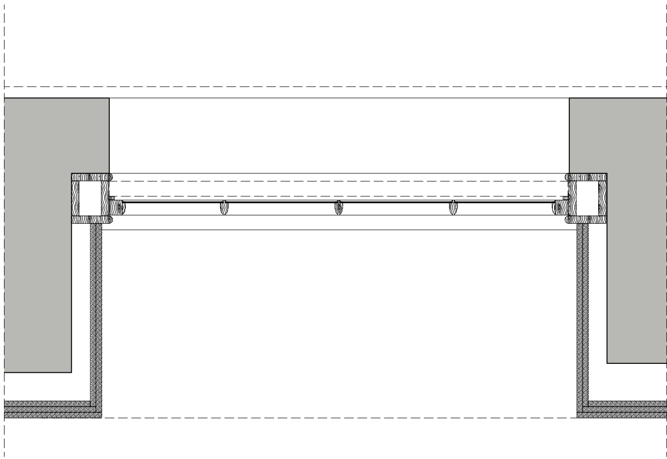
3 Proposed Internal Elevation 1:10@A1
