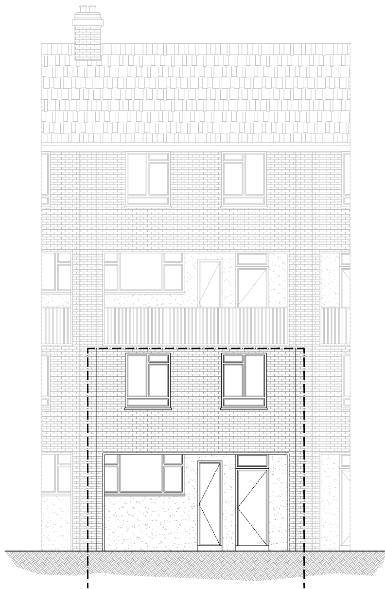
FRONT ELEVATION AS APPROVED
