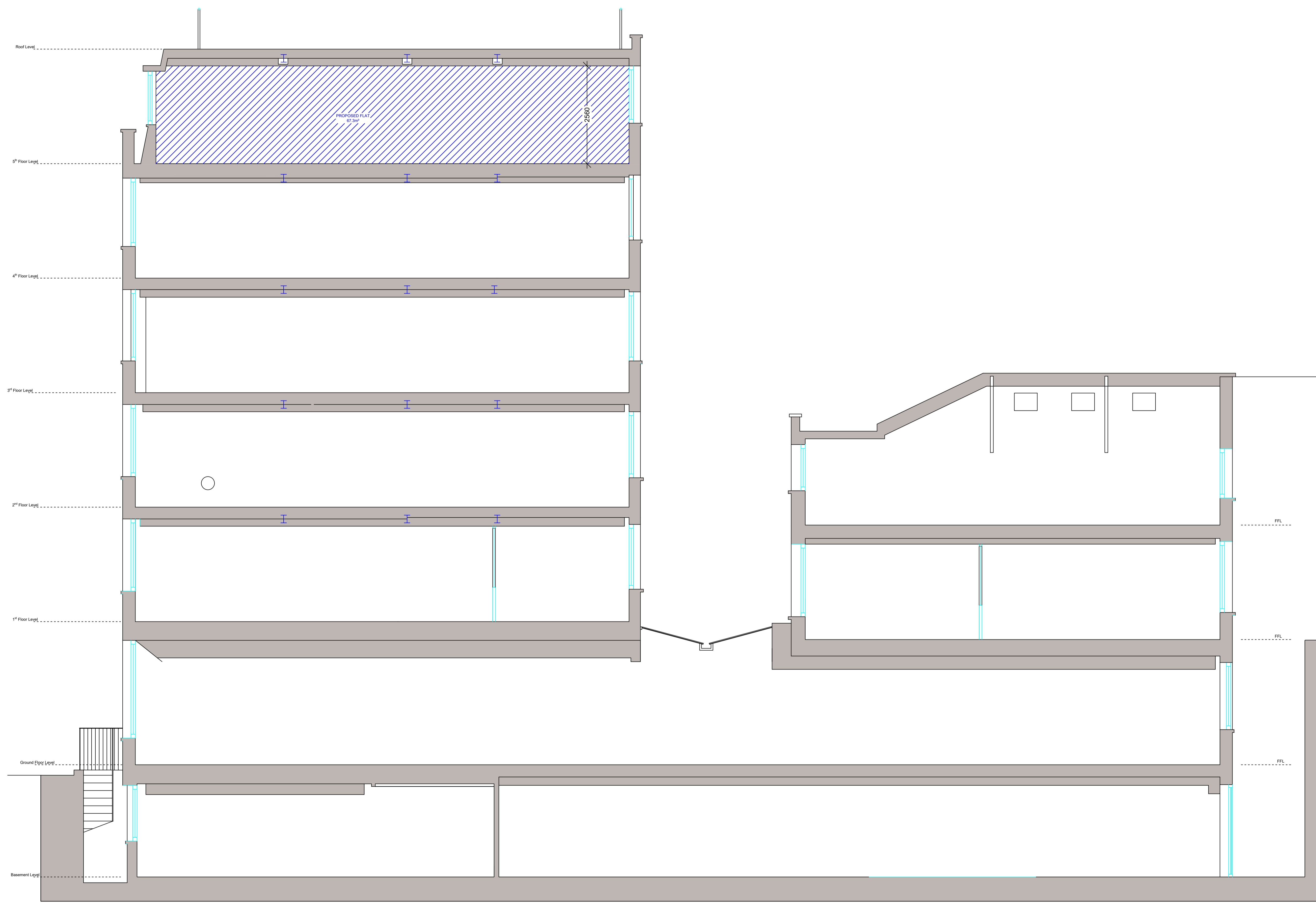
○ Cross Section 1: 50
