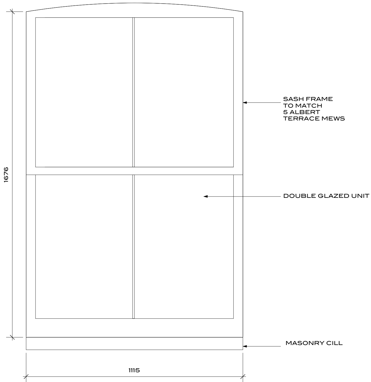
FRONT ELEVATION
