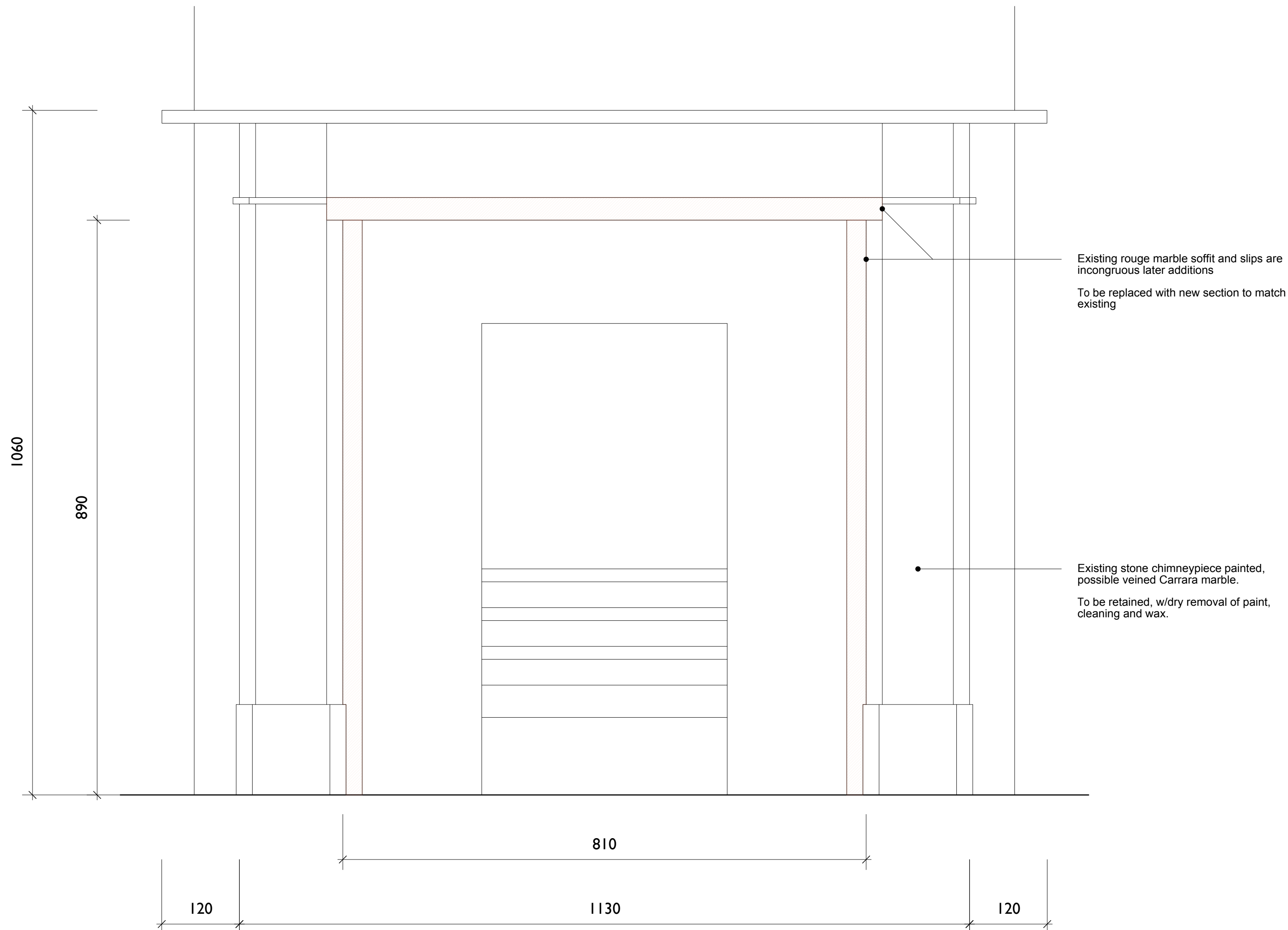
1 Existing Elevation 1:5@A1
