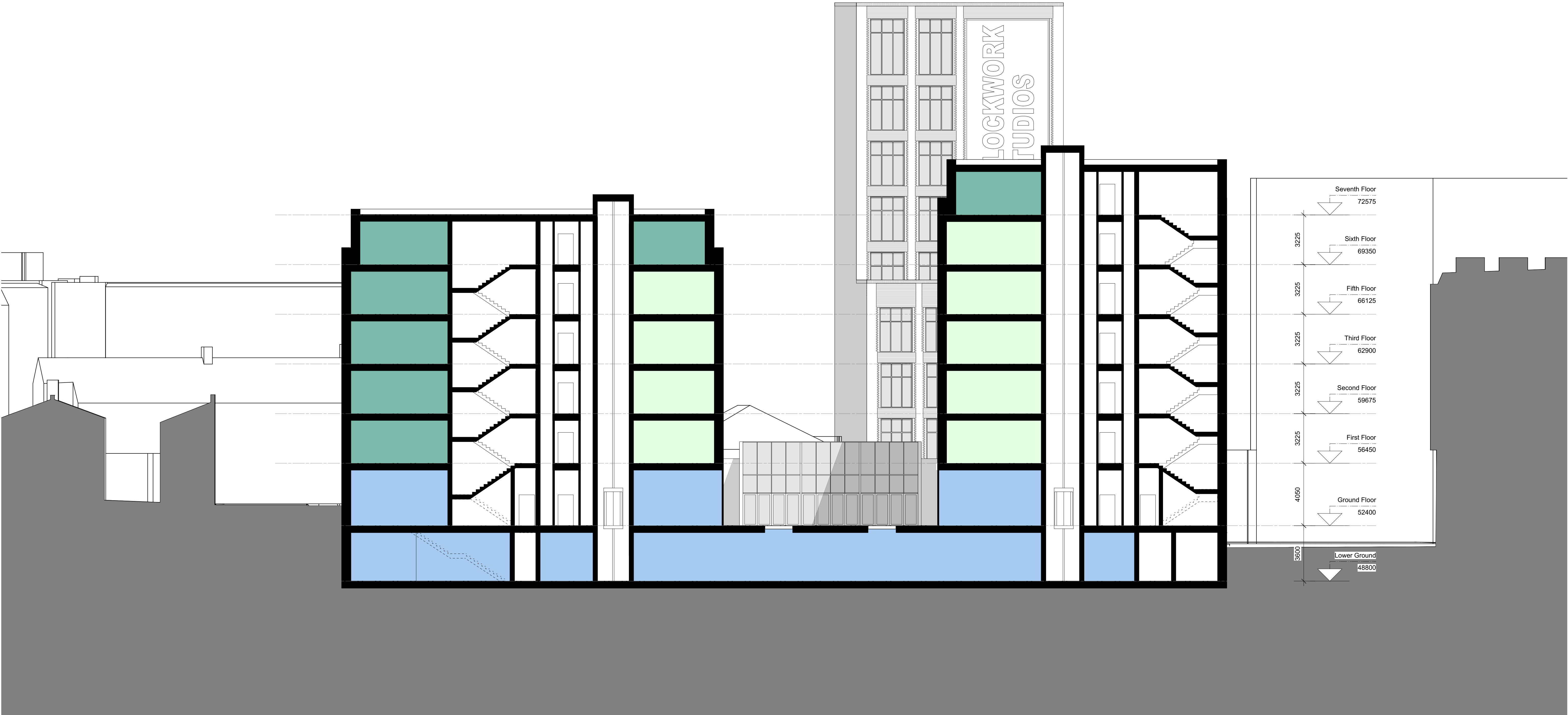
1 SECTION AA - PROPOSED Scale: 1:125
