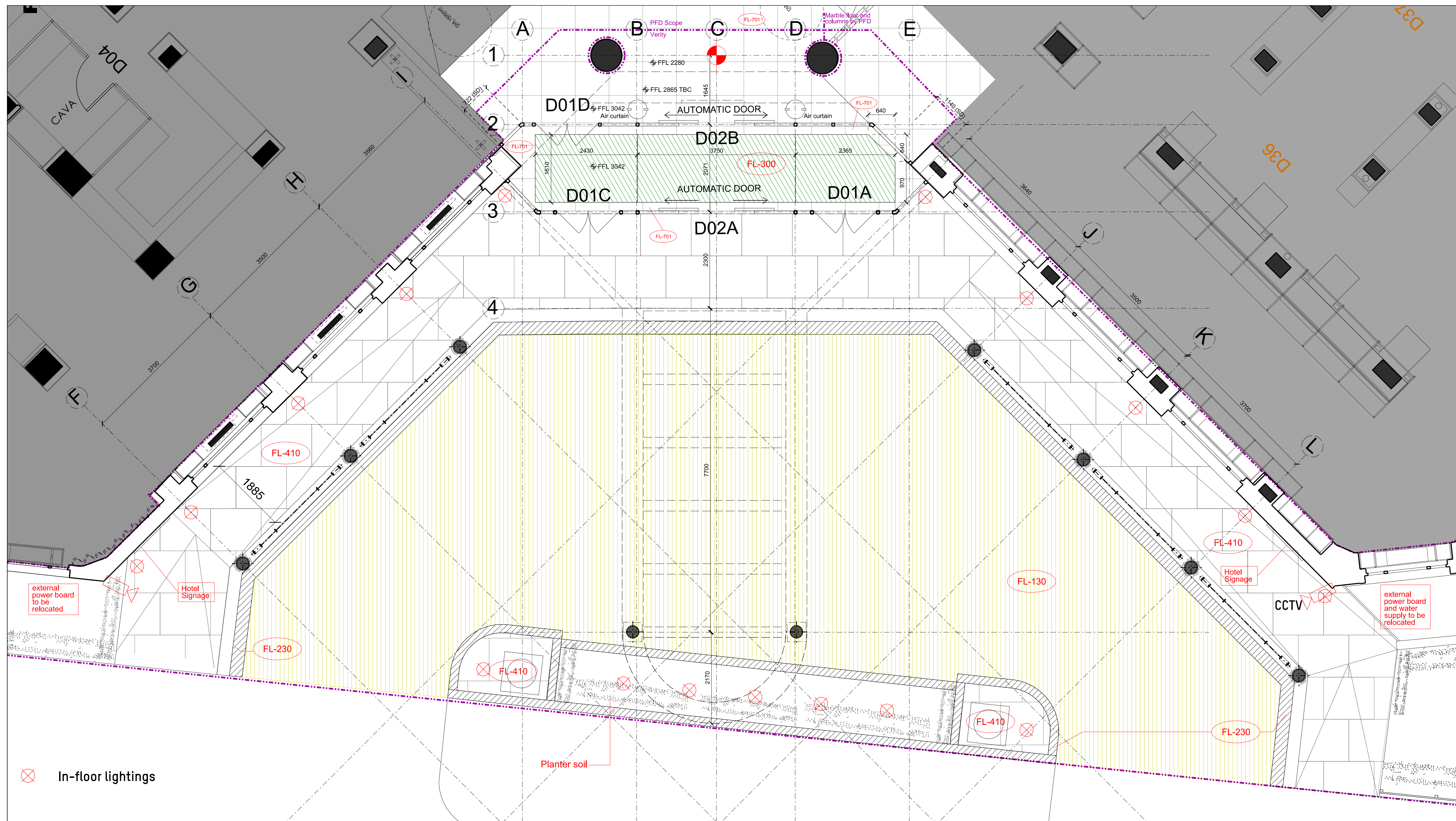
PROPOSED- PLAN
