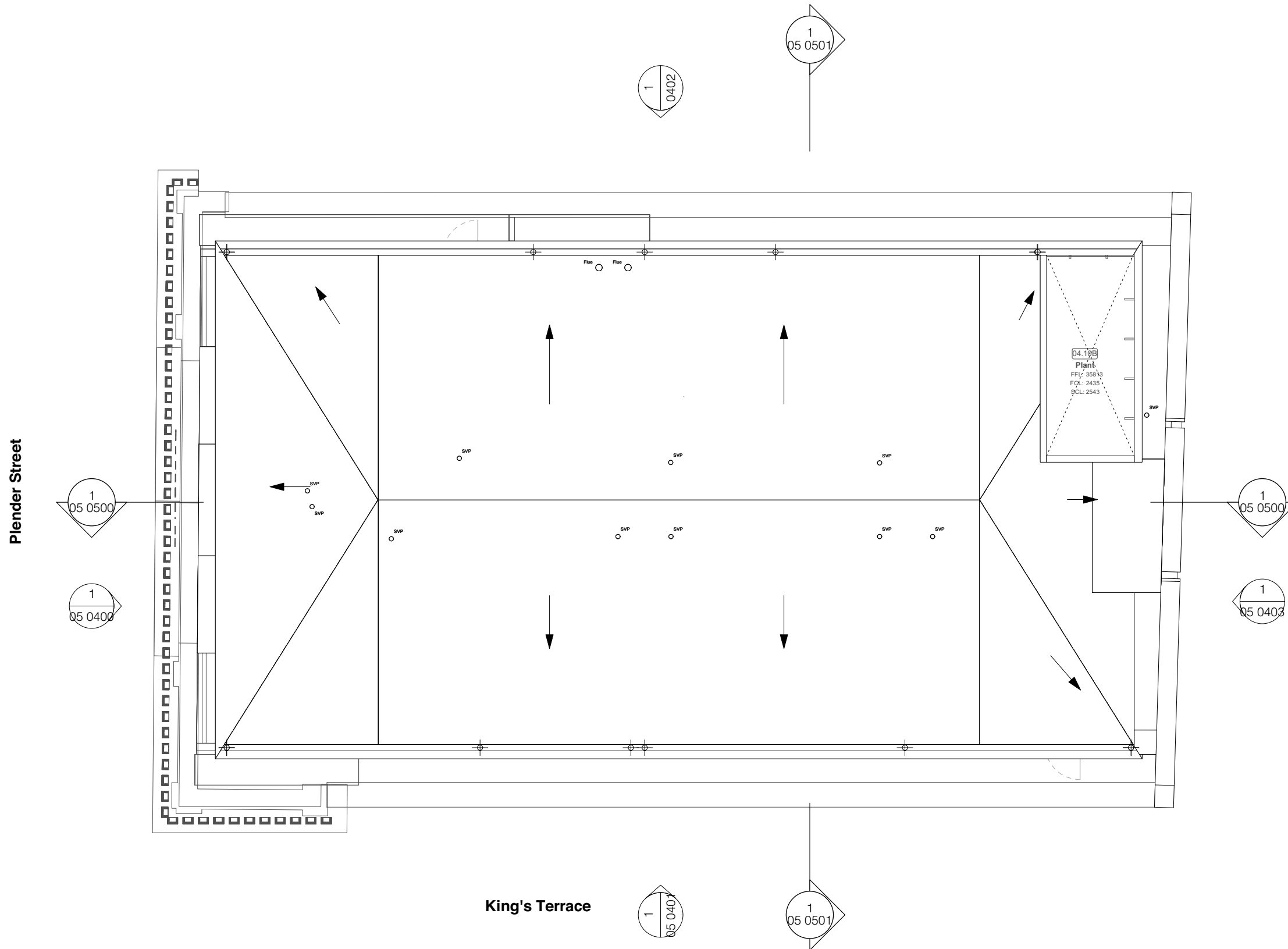
1 Proposed Roof Plan Scale: 1:100
