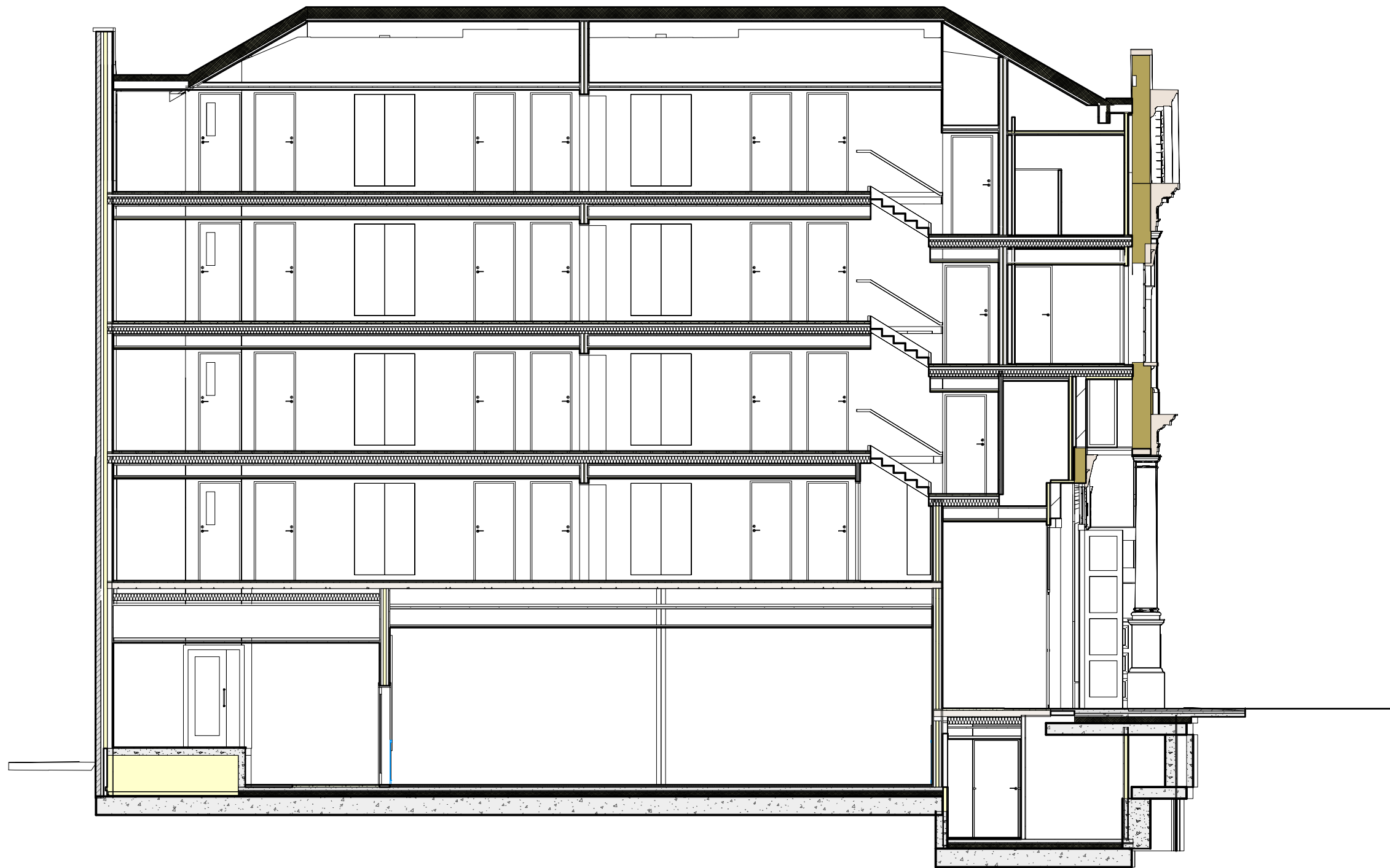
1 Proposed Long Section Scale: 1:100
