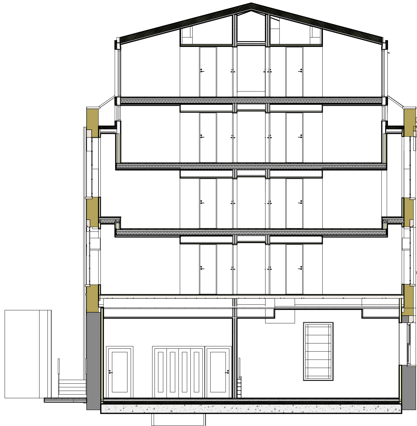
1 Proposed Short Section Scale: 1:100
