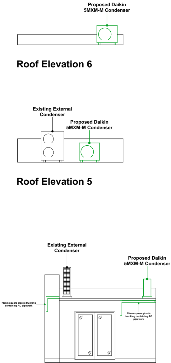
Courtyard Elevation 3
