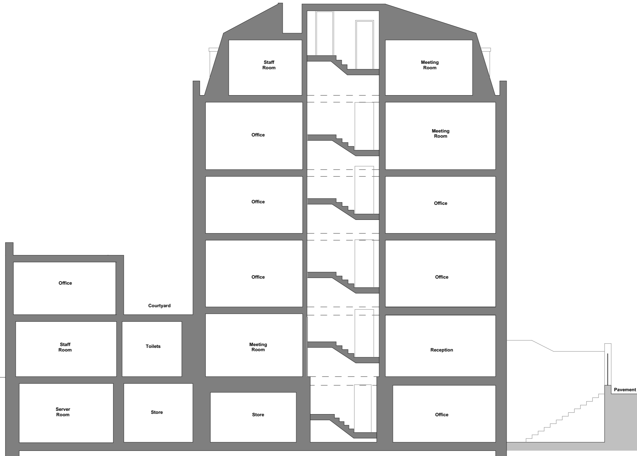
Section - S01
