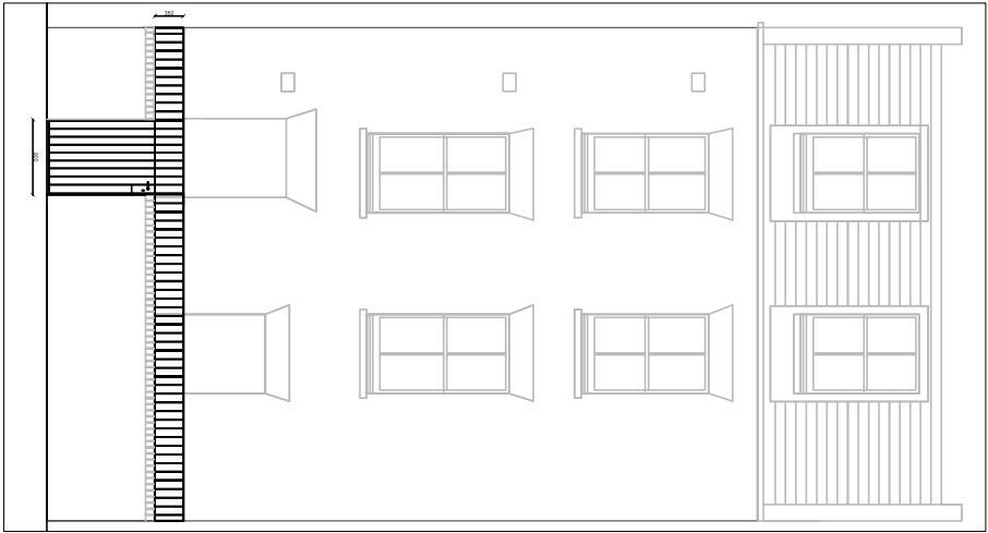
Front Elevation 1 to 100
